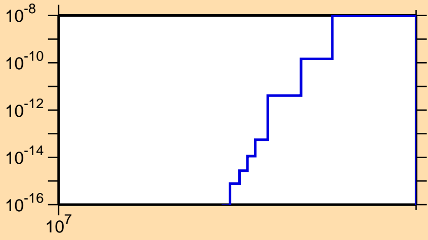
\sigma vs. E for ^{150}\text{Dy}(n,pt)
