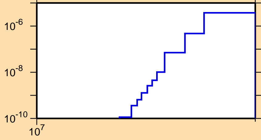
\sigma vs. E for ^{150}\text{Dy}(n,2n\alpha)
