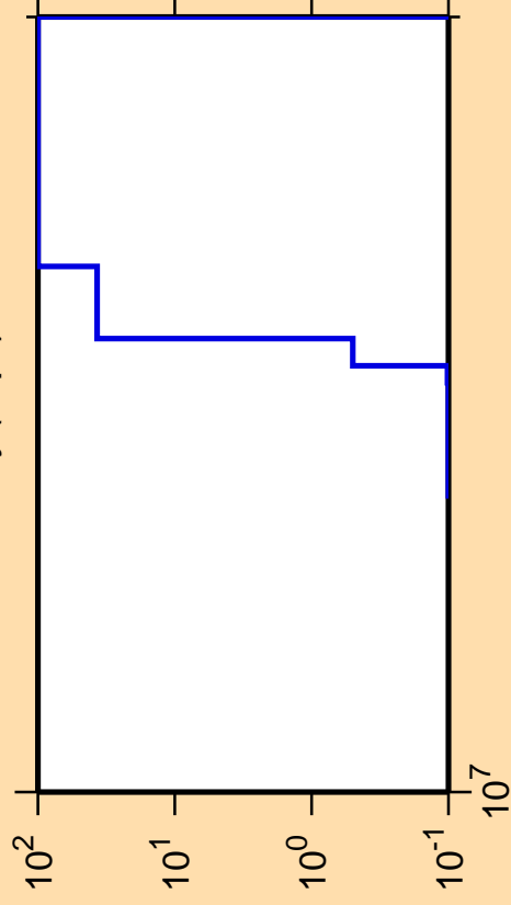
\Delta\sigma/\sigma vs. E for ^{150}\text{Dy}(n,pt)
