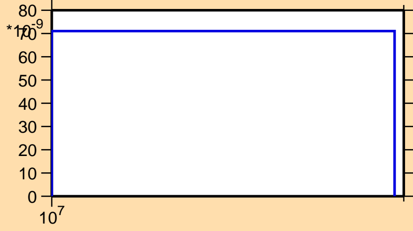
\sigma vs. E for ^{150}\text{Dy}(n,2n\alpha)
