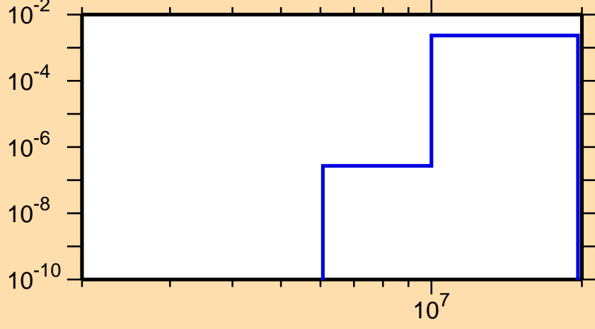
\sigma vs. E for ^{150}\text{Dy}(n,d)
