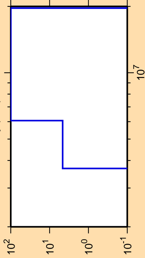
\Delta\sigma/\sigma vs. E for ^{150}\text{Dy}(n,d)
