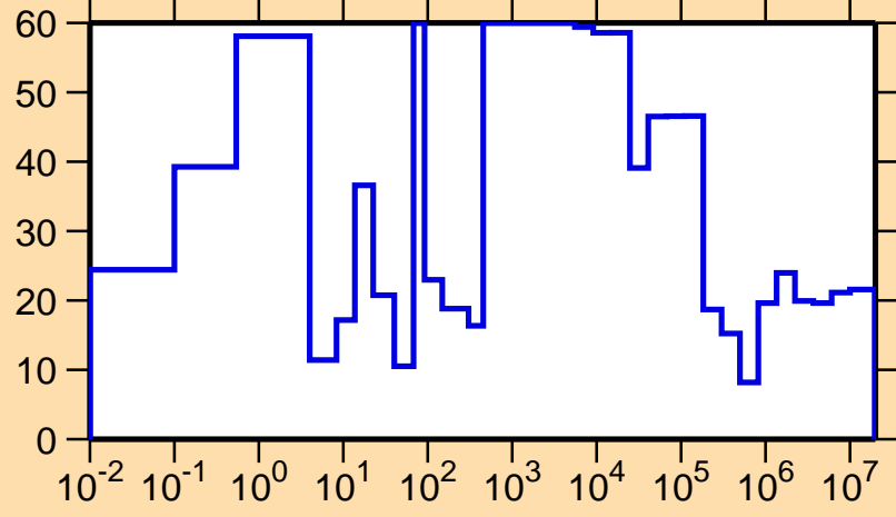
\Delta\sigma/\sigma vs. E for ^{150}\text{Dy}(n,tot.)
