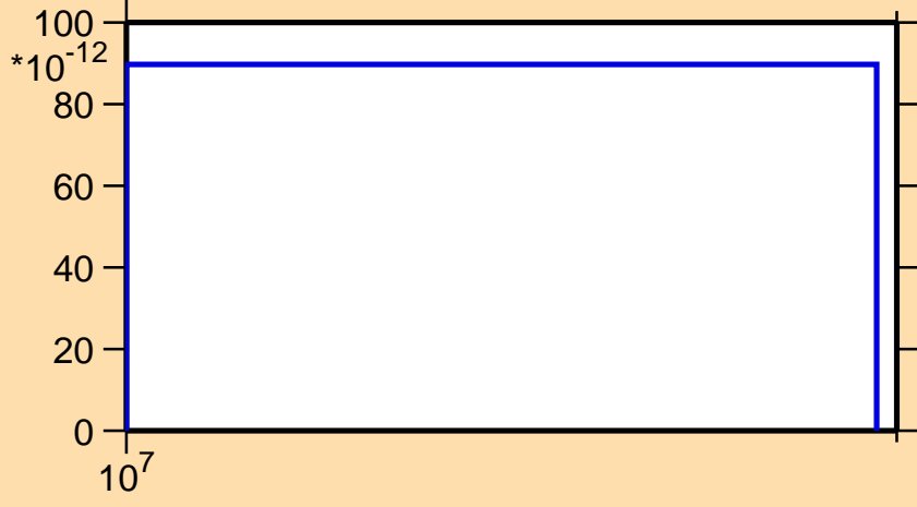
\sigma vs. E for ^{150}\text{Dy}(n,pt)
