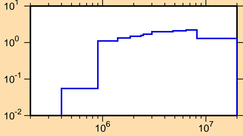
\sigma vs. E for ^{150}\text{Dy}(n,\text{inel.})
