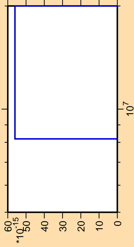
\Delta\sigma/\sigma vs. E for ^{150}\text{Dy} (mt 11)
