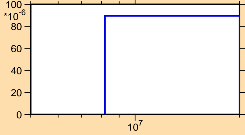
\sigma vs. E for ^{150}\text{Dy}(n,t)
