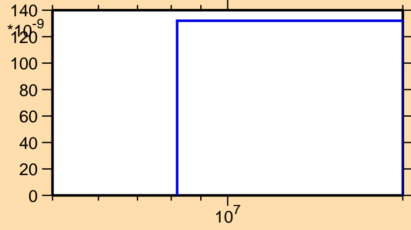
\sigma vs. E for ^{150}\text{Dy} (mt 45)
