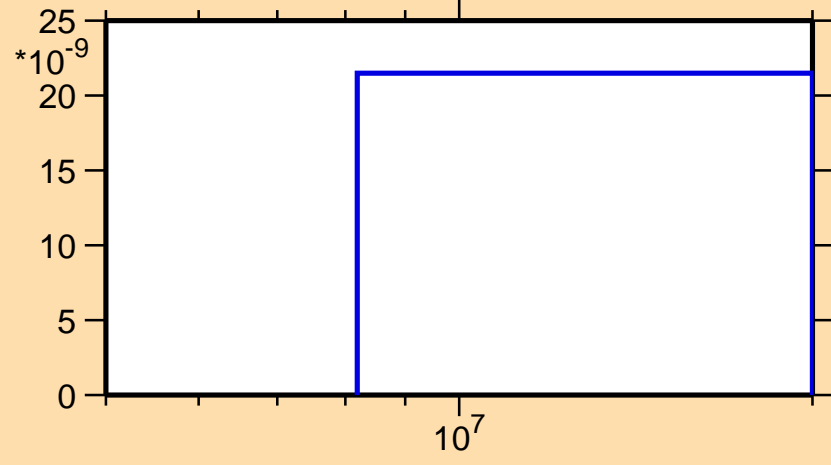
\sigma vs. E for ^{150}\text{Dy}(n,\text{nd})
