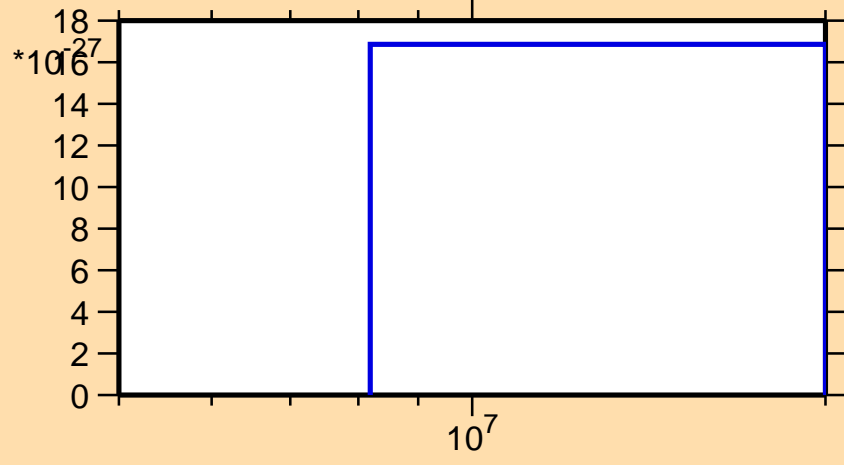
\sigma vs. E for ^{150}\text{Dy} (mt 11)
