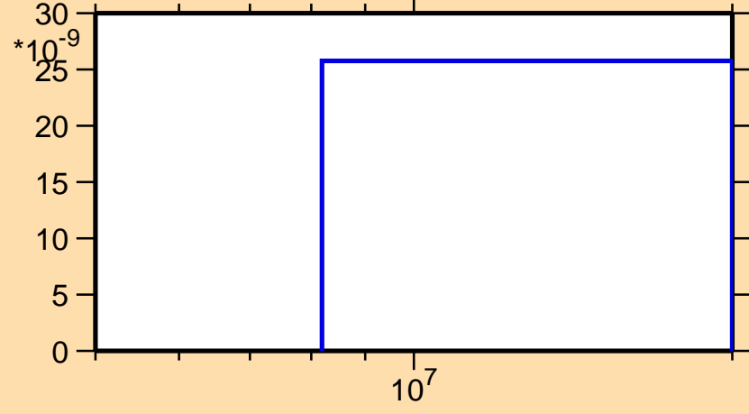
\sigma vs. E for ^{150}\text{Dy}(n,\text{pd})
