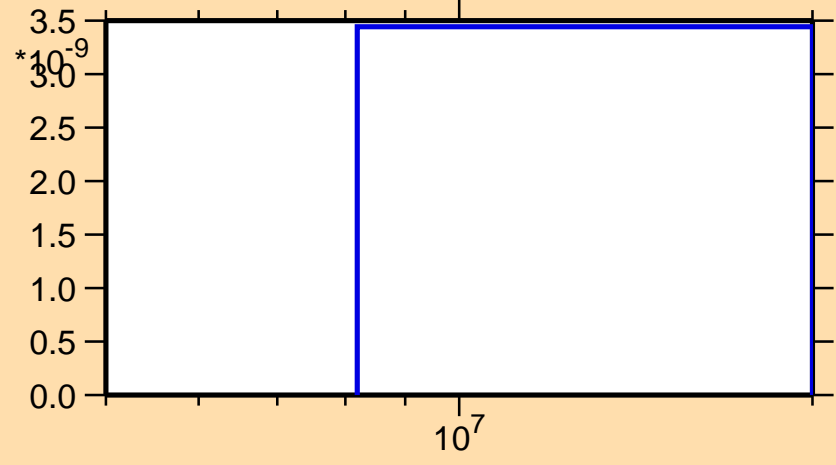
\sigma vs. E for ^{150}\text{Dy}(\text{mt117})
