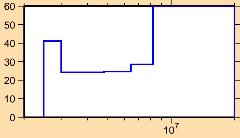
\Delta\sigma/\sigma vs. E for ^{150}\text{Dy}(n,ncont.)
