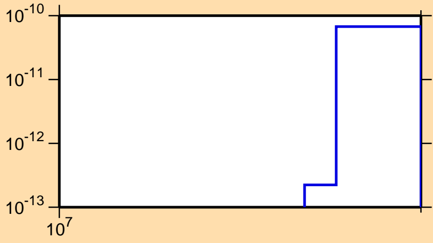
\sigma vs. E for ^{152}\text{Dy}(n,\text{pt})
