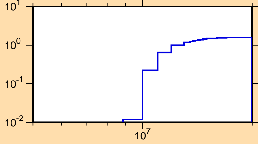
\sigma vs. E for ^{152}\text{Dy}(n,2n)
