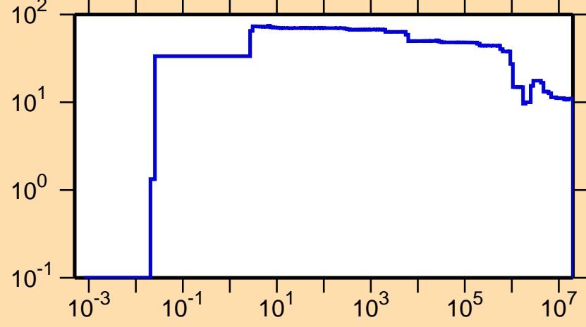
\Delta\sigma/\sigma vs. E for ^{152}\text{Dy}(n,\text{nonel.})
