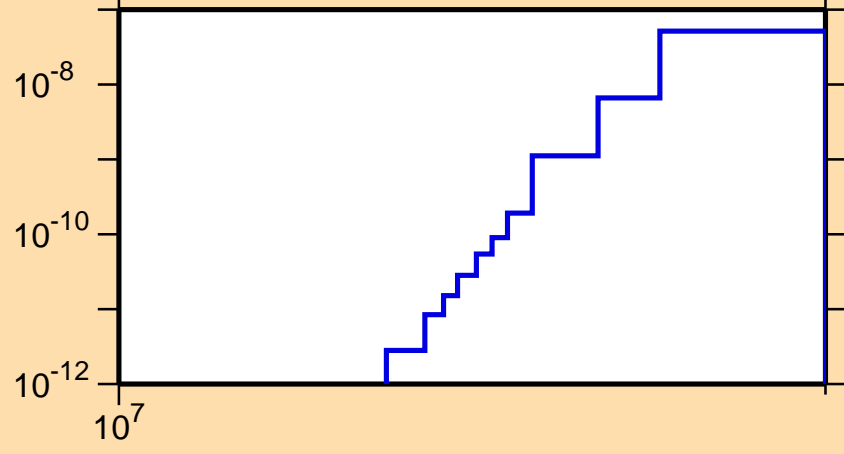
\sigma vs. E for ^{152}\text{Dy} (mt 45)
