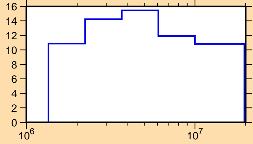
\Delta\sigma/\sigma vs. E for ^{152}\text{Dy}(n,n\text{nonel.})
