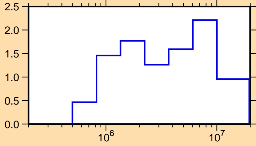
\sigma vs. E for ^{152}\text{Dy}(n,\text{inel.})
