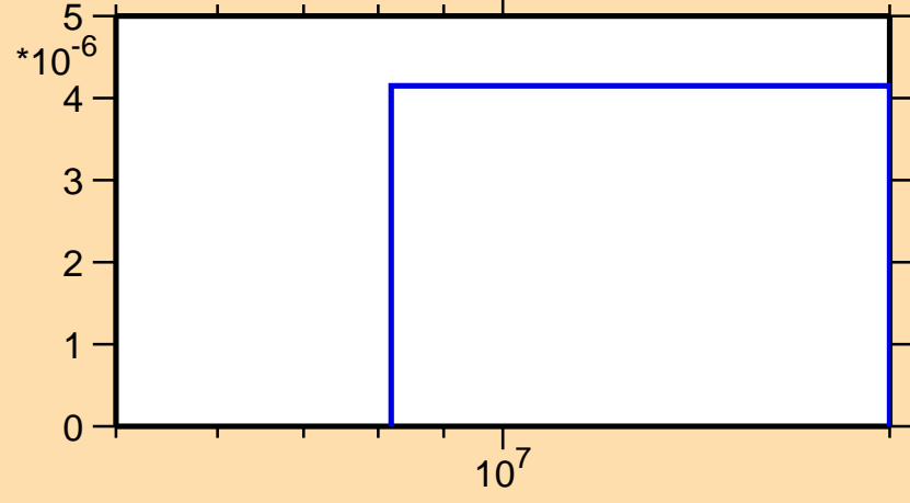
\sigma vs. E for ^{152}\text{Dy}(n,2n\alpha)
