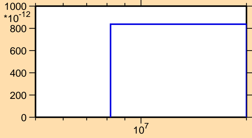
\sigma vs. E for ^{152}\text{Dy}(\text{mt } 45)
