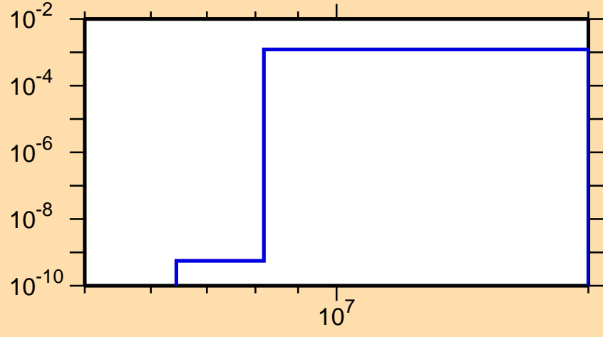
\sigma vs. E for ^{152}\text{Dy}(n,d)
