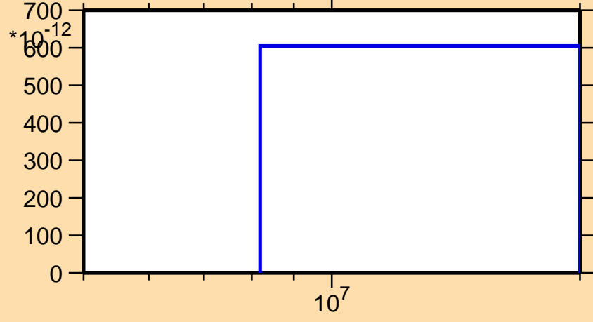
\sigma vs. E for ^{152}\text{Dy}(n,3n\alpha)
