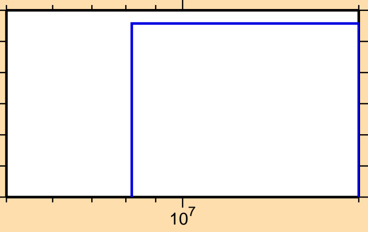
\sigma vs. E for ^{152}\text{Dy}(n,\text{pt})
