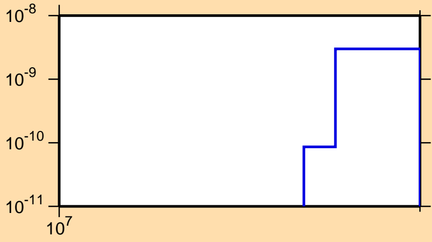
\sigma vs. E for ^{153}\text{Dy}(n,\text{pt})
