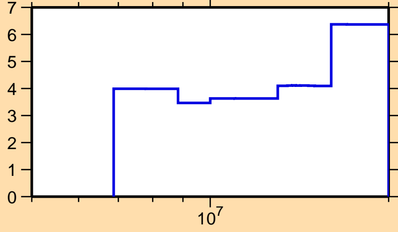
\Delta\sigma/\sigma vs. E for ^{153}\text{Dy}(n,\text{tot.})
