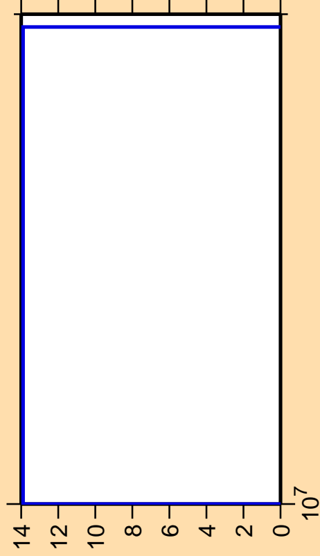
\Delta\sigma/\sigma vs. E for ^{153}\text{Dy}(n,\text{pd})
