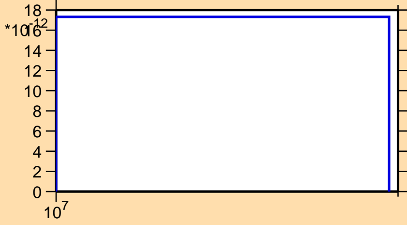
\sigma vs. E for ^{153}\text{Dy}(n,\text{pd})
