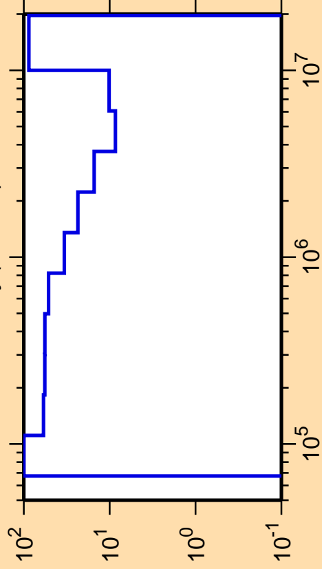
\Delta\sigma/\sigma vs. E for ^{153}\text{Dy}(n,\text{inel.})
