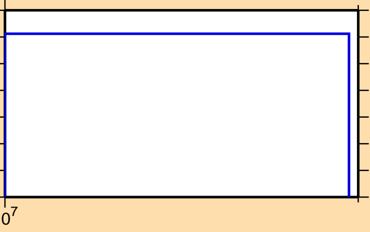
\sigma vs. E for ^{153}\text{Dy}(n,3n)
