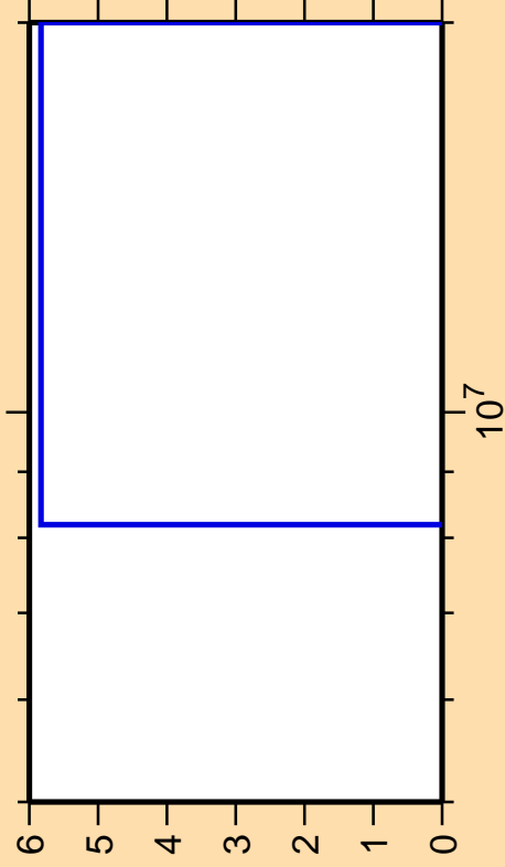
\Delta\sigma/\sigma vs. E for ^{153}\text{Dy}(\text{mt } 34)
