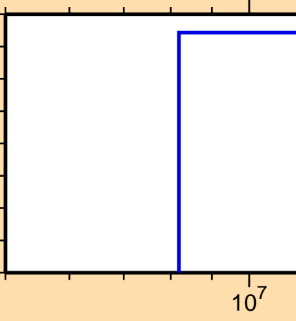
\sigma vs. E for ^{153}\text{Dy}(n,\text{pd})
