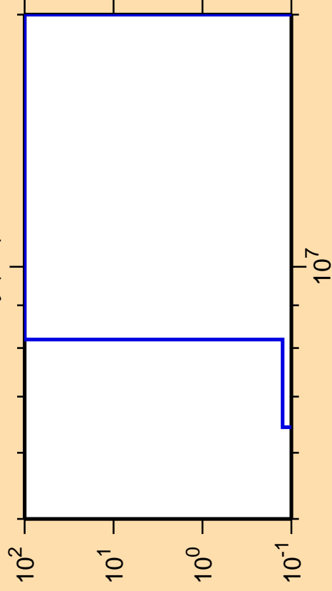
\Delta\sigma/\sigma vs. E for ^{153}\text{Dy}(n,t)
