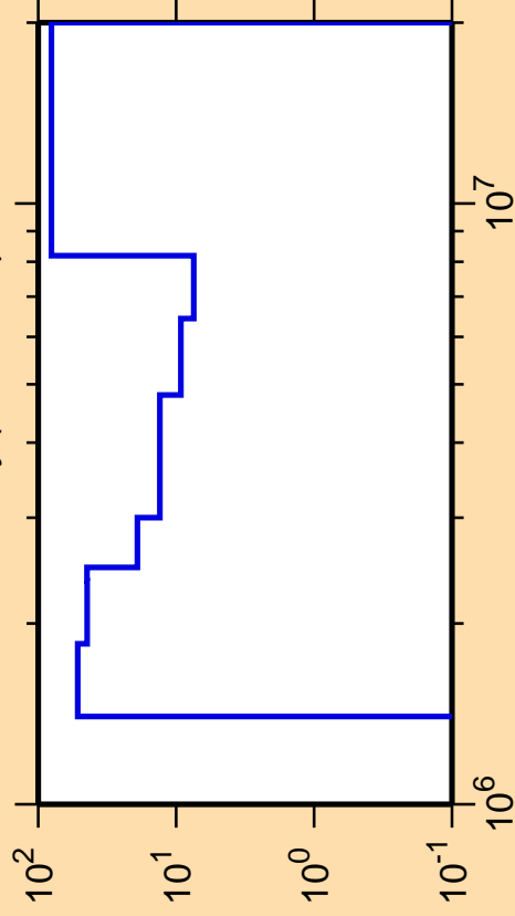
\Delta\sigma/\sigma vs. E for ^{153}\text{Dy}(n,\text{ncont.})
