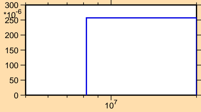
\sigma vs. E for ^{153}\text{Dy}(n,3n)
