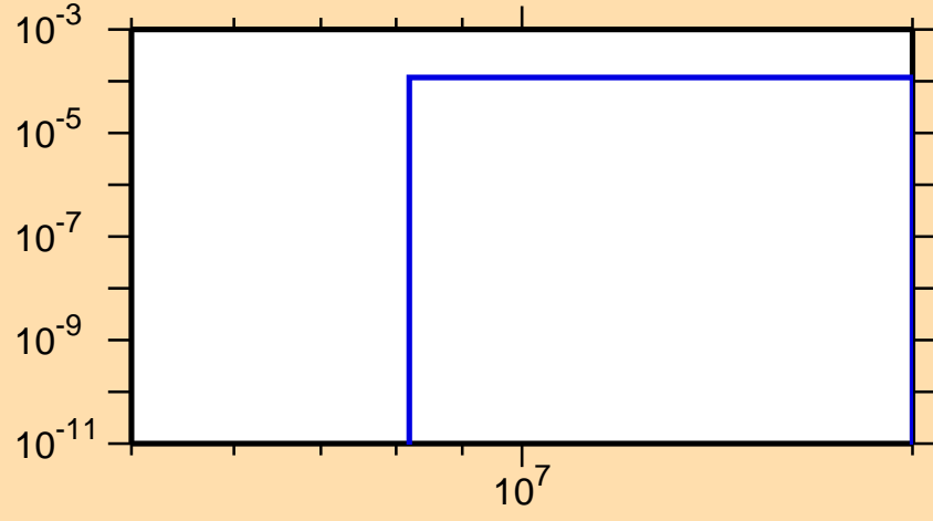
\sigma vs. E for ^{153}\text{Dy}(n,t)
