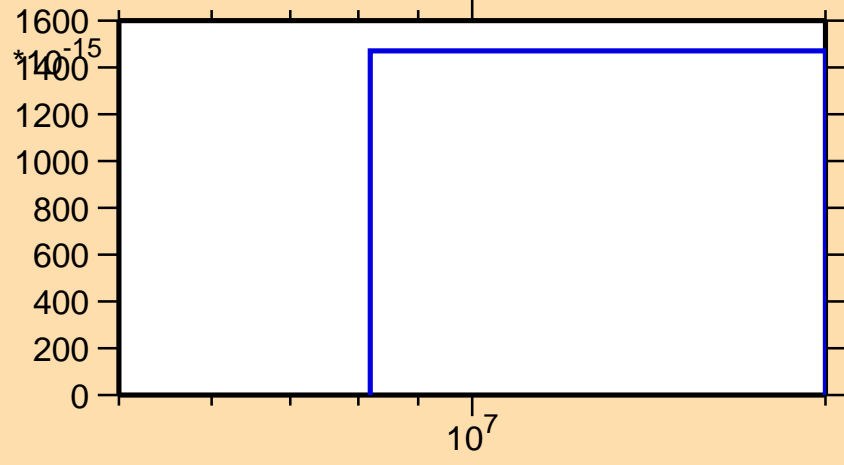
\sigma vs. E for ^{153}\text{Dy}(\text{mt } 34)
