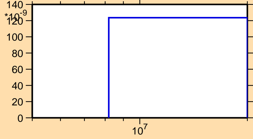
\sigma vs. E for ^{153}\text{Dy}(n,\text{nd})
