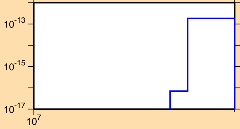
\sigma vs. E for ^{154}\text{Dy} (mt 34)
