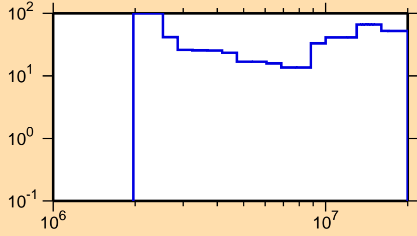
\Delta\sigma/\sigma vs. E for ^{154}\text{Dy}(n,ncont.)
