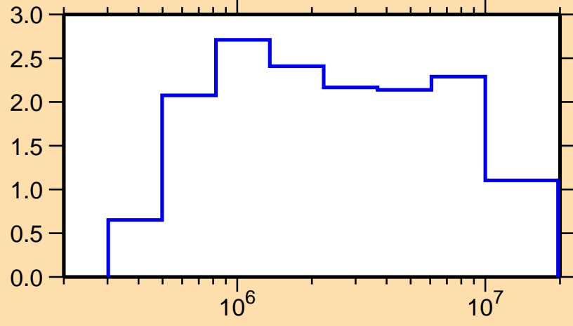
\sigma vs. E for ^{154}\text{Dy}(n,\text{inel.})
