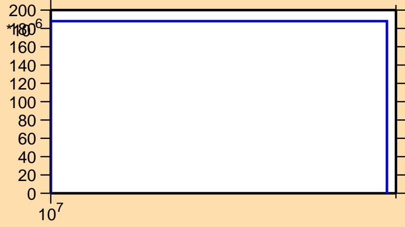
\sigma vs. E for ^{154}\text{Dy}(n,3n)
