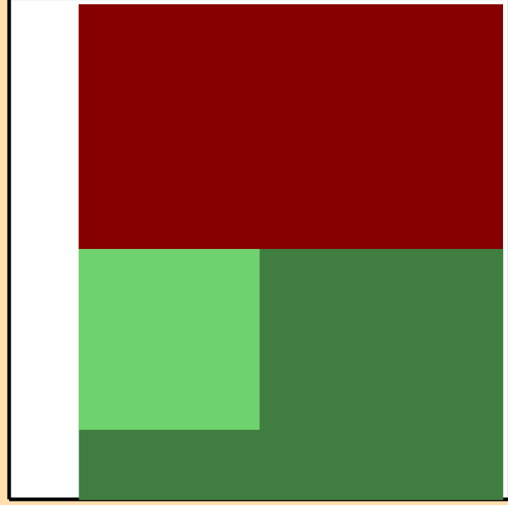
\Delta\sigma/\sigma vs. E for ^{154}\text{Dy}(n,2n)
