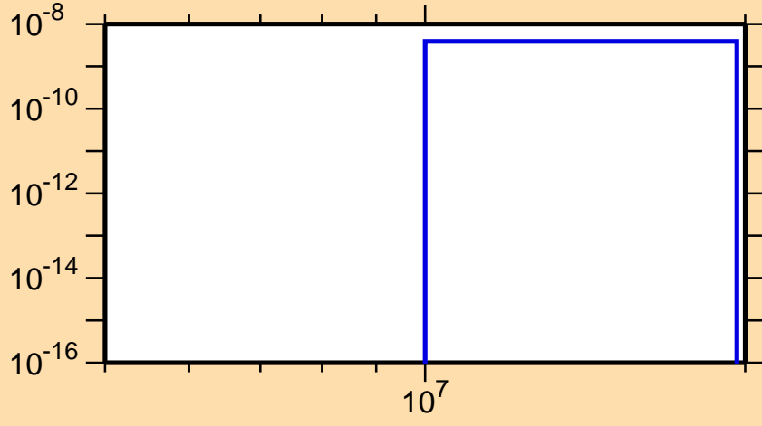
\sigma vs. E for ^{154}\text{Dy}(n,\text{He3})
