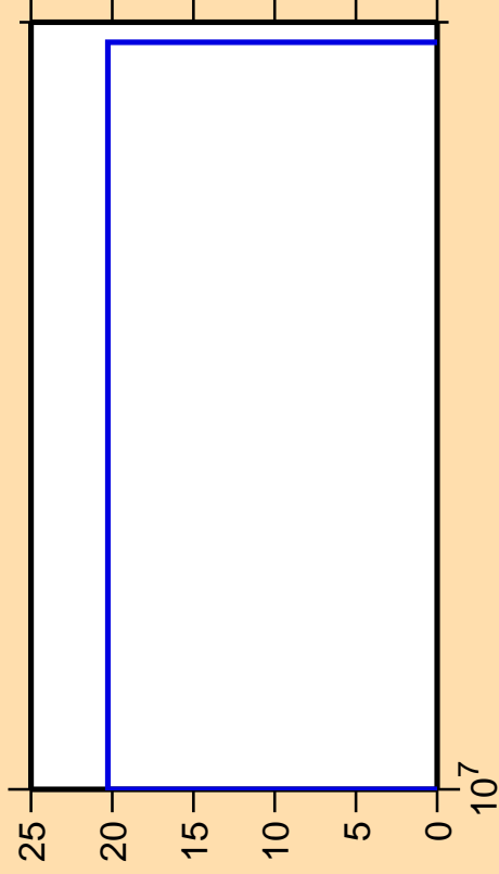
\Delta\sigma/\sigma vs. E for ^{154}\text{Dy}(n,\text{pd})
