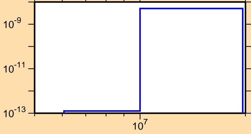
\sigma vs. E for ^{154}\text{Dy}(n,p\alpha)
