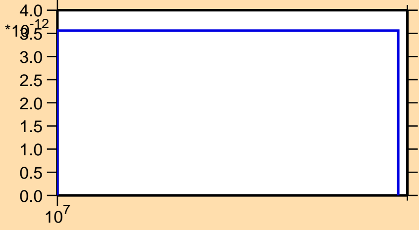
\sigma vs. E for ^{154}\text{Dy}(n,\text{pd})
