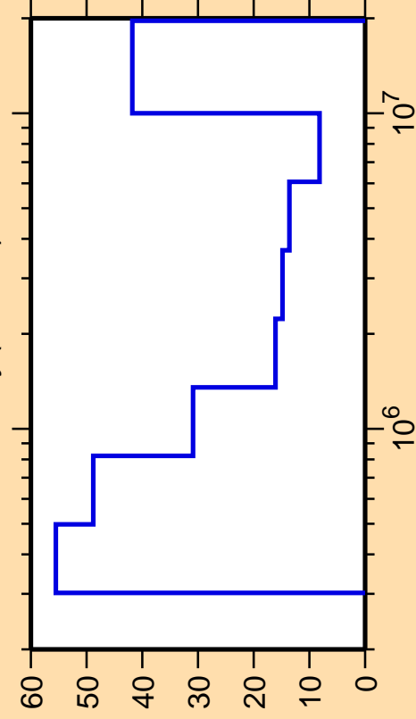
\Delta\sigma/\sigma vs. E for ^{154}\text{Dy}(n,\text{inel.})
