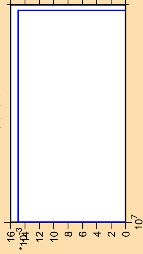
\Delta\sigma/\sigma vs. E for ^{154}\text{Dy}(n,\text{pt})
