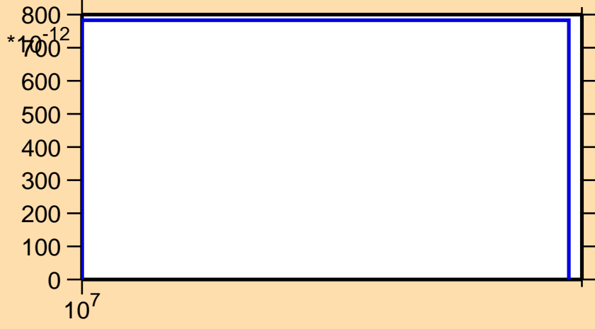
\sigma vs. E for ^{154}\text{Dy}(n,\text{nd})
