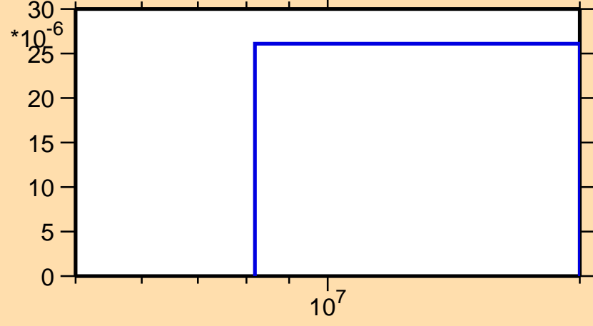
\sigma vs. E for ^{154}\text{Dy}(n,t)
