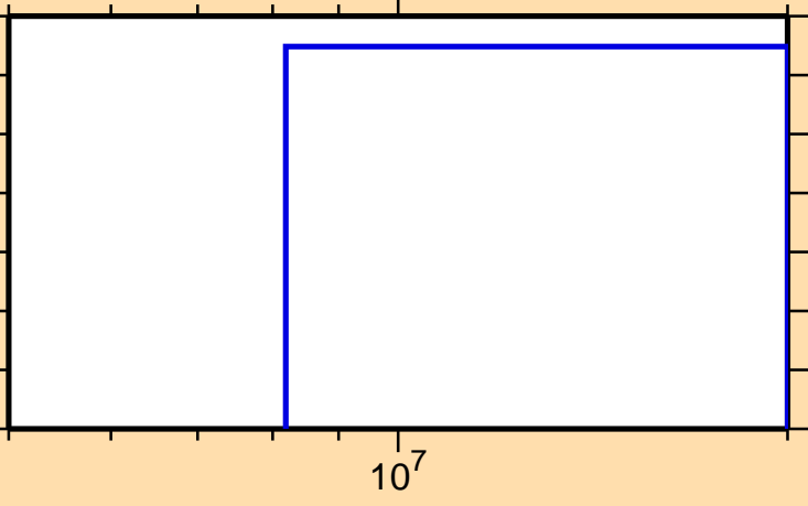
\sigma vs. E for ^{154}\text{Dy}(n,\text{He3})
