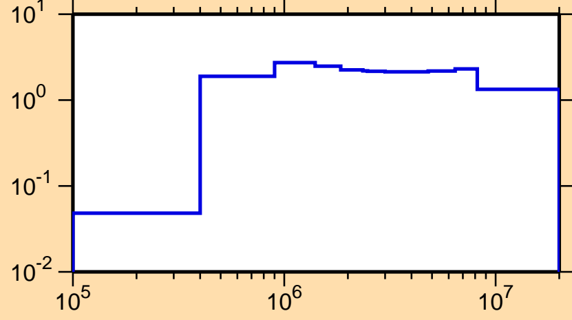
\sigma vs. E for ^{154}\text{Dy}(n,\text{inel.})
