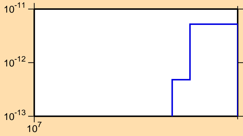
\sigma vs. E for ^{155}\text{Dy} (mt117)
