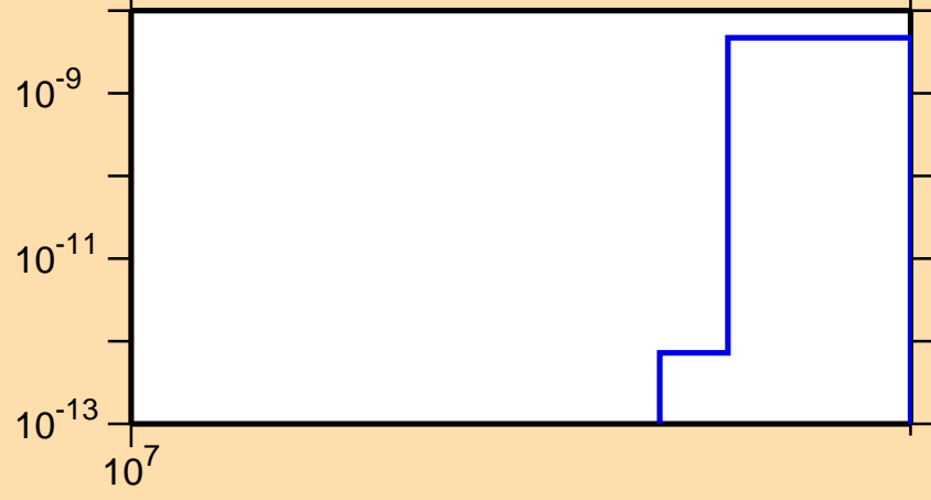
\sigma vs. E for ^{155}\text{Dy}(n,nt)
