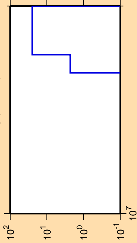
\Delta\sigma/\sigma vs. E for ^{155}\text{Dy} (mt117)
