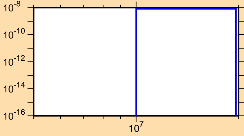
\sigma vs. E for ^{155}\text{Dy}(n,\text{He3})
