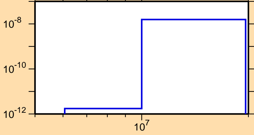
\sigma vs. E for ^{155}\text{Dy}(n,p\alpha)
