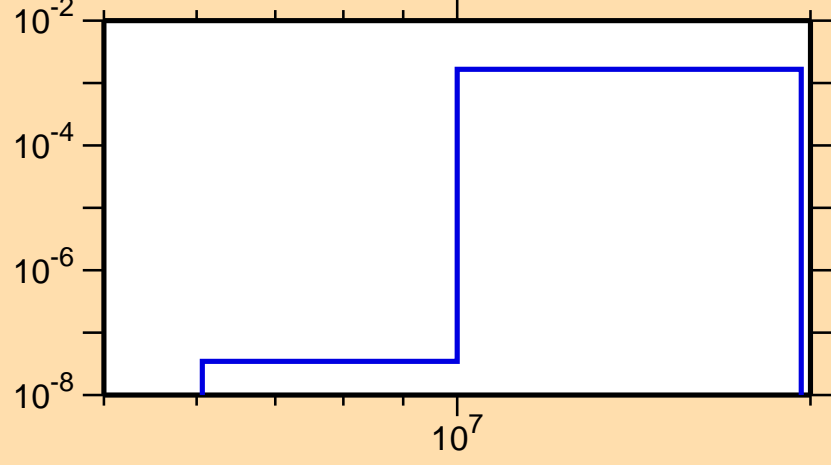
\sigma vs. E for ^{155}\text{Dy}(n,d)
