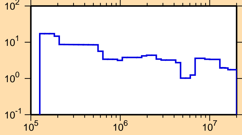
\Delta\sigma/\sigma vs. E for ^{156}\text{Dy}(n,\text{tot.})
