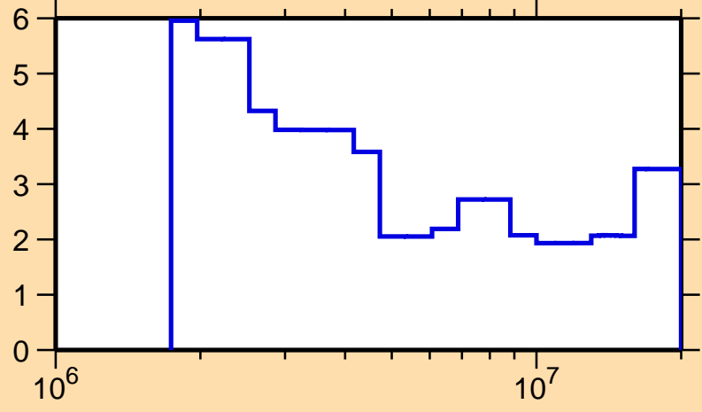
\Delta\sigma/\sigma vs. E for ^{156}\text{Dy}(n,n\text{onel.})
