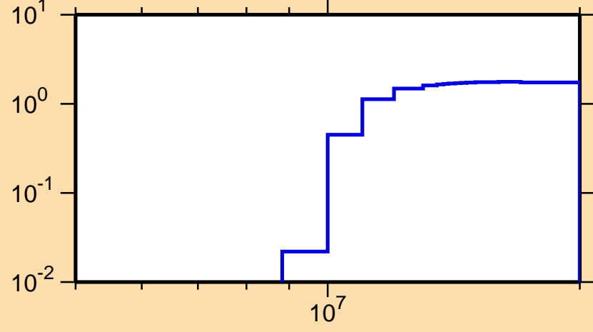
\sigma vs. E for ^{156}\text{Dy}(n,2n)
