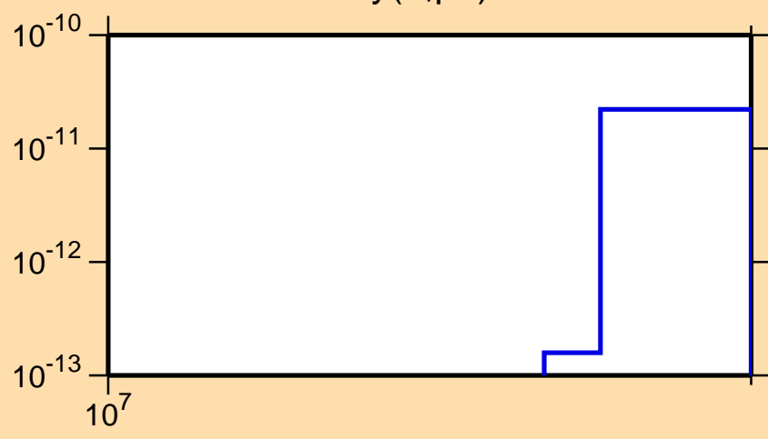
\sigma vs. E for ^{156}\text{Dy}(n,pd)
