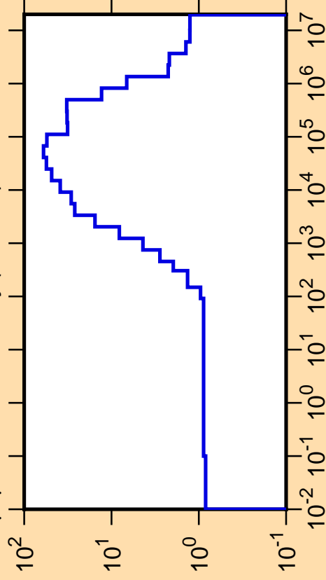
\Delta\mu/\mu vs. E for ^{156}\text{Dy}(\text{mt251})
