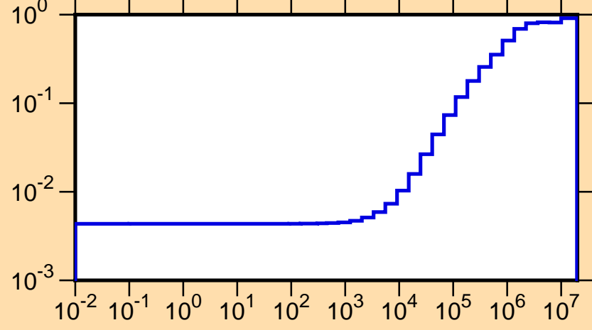
\mu vs. E for ^{156}\text{Dy}(\text{mt251})
