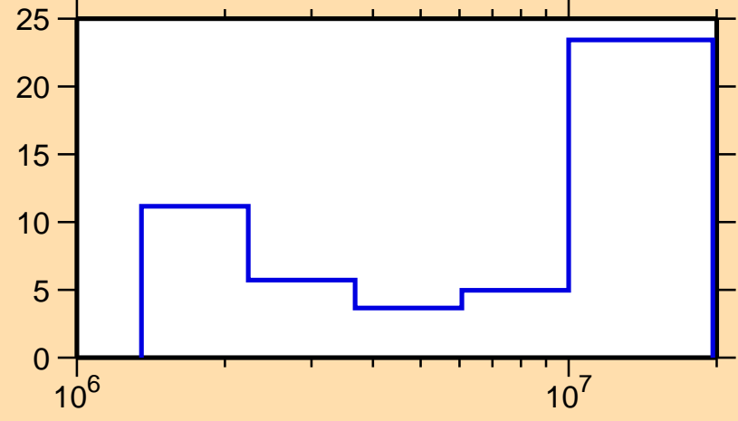
\Delta\sigma/\sigma vs. E for ^{156}\text{Dy}(n,ncont.)
