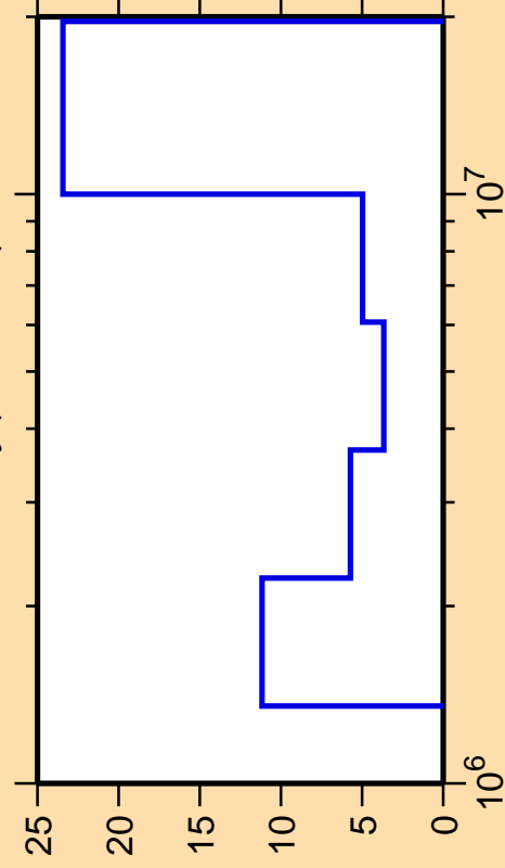
\Delta\sigma/\sigma vs. E for ^{156}\text{Dy}(n,\text{ncont.})
