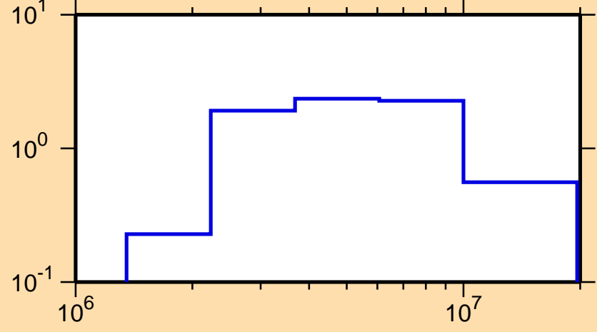
\sigma vs. E for ^{156}\text{Dy}(n,ncont.)
