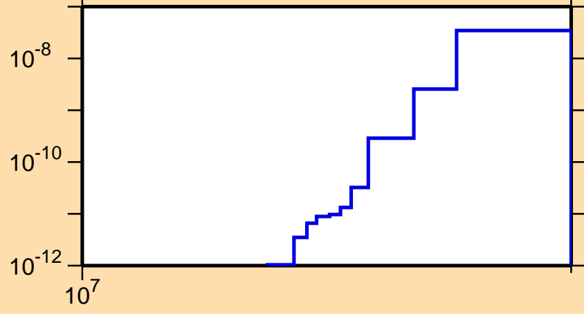
\sigma vs. E for ^{157}\text{Dy}(n,\text{He3})
