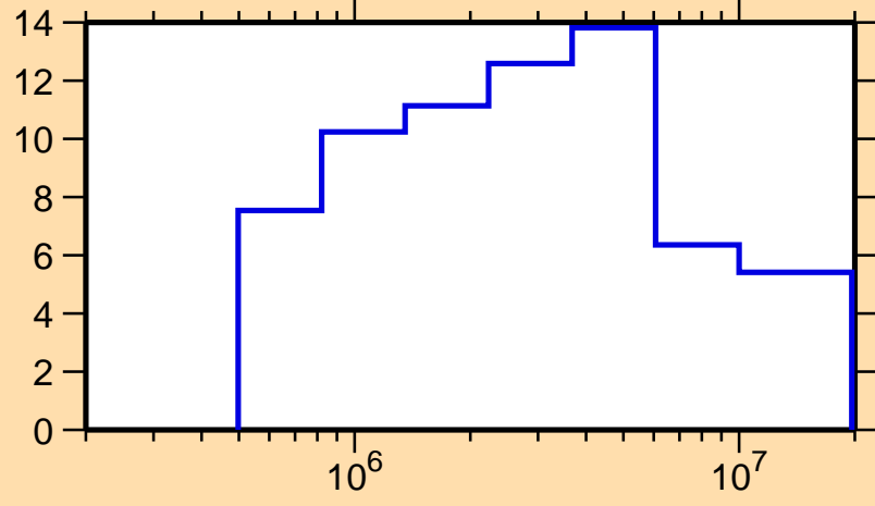
\Delta\sigma/\sigma vs. E for ^{157}\text{Dy}(n,el.)
