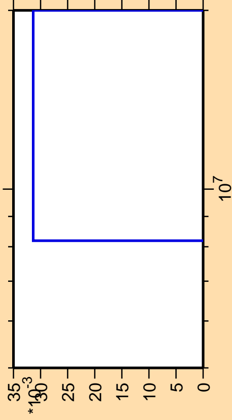
\Delta\sigma/\sigma vs. E for ^{157}\text{Dy} (mt 34)
