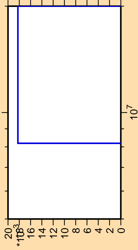
\Delta\sigma/\sigma vs. E for ^{157}\text{Dy}(n,\text{pd})
