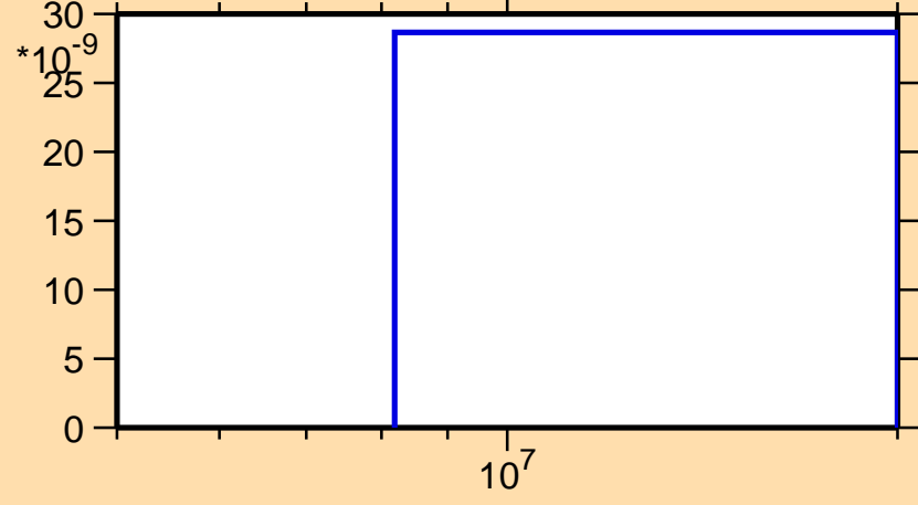
\sigma vs. E for ^{157}\text{Dy}(n,2np)
