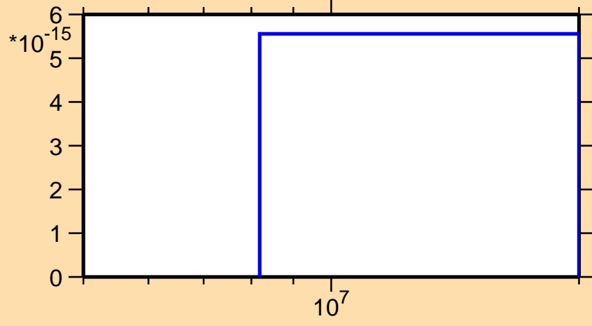
\sigma vs. E for ^{157}\text{Dy} (mt 34)
