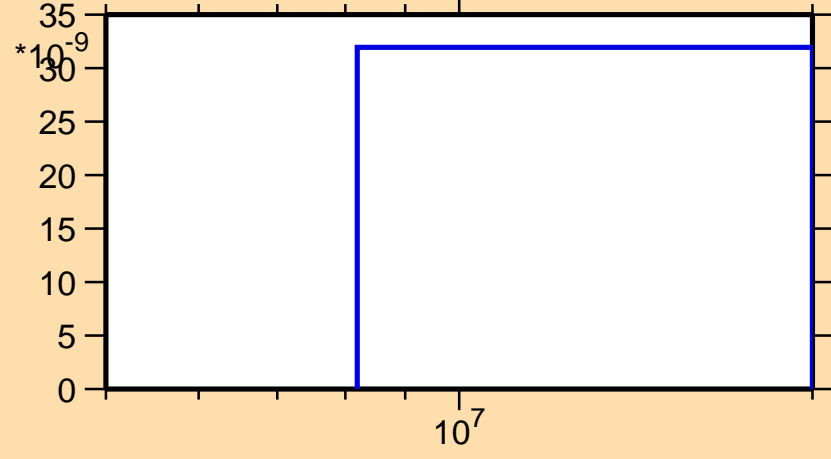
\sigma vs. E for ^{157}\text{Dy}(n,\text{nd})
