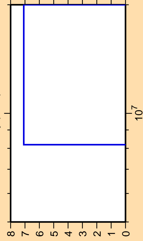
\Delta\sigma/\sigma vs. E for ^{157}\text{Dy}(n,nt)
