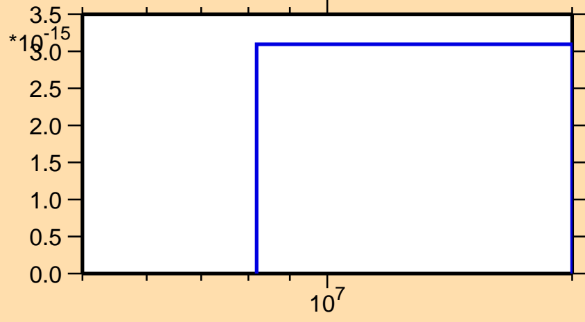
\sigma vs. E for ^{157}\text{Dy}(n,\text{pd})
