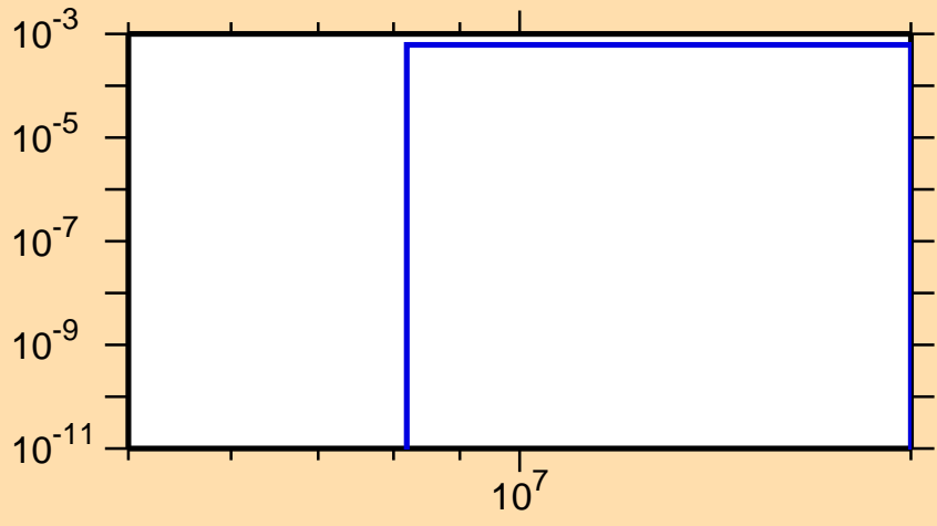
\sigma vs. E for ^{157}\text{Dy}(n,np)
