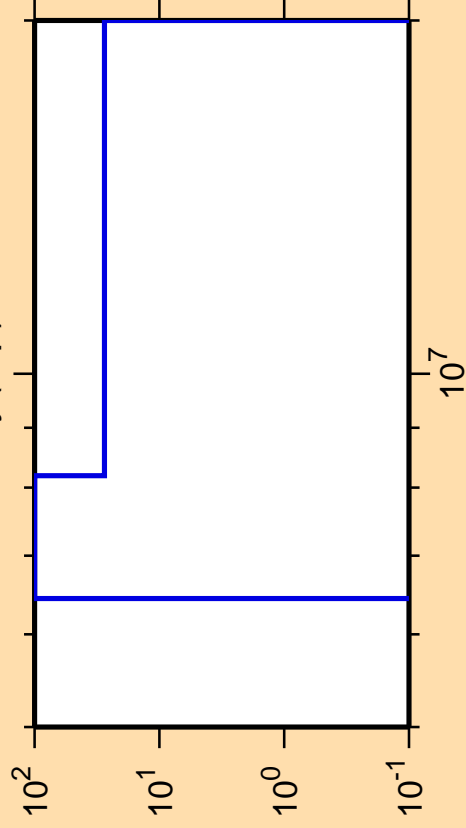
\Delta\sigma/\sigma vs. E for ^{157}\text{Dy}(n,p)
