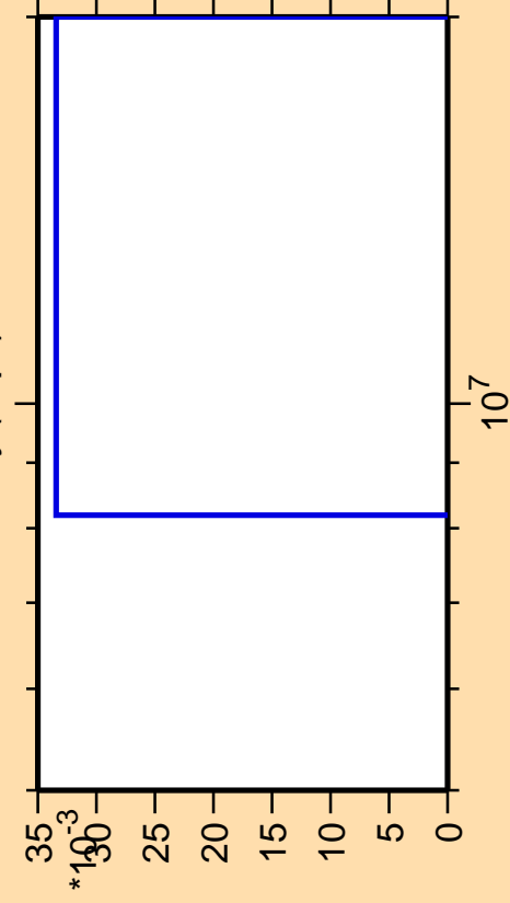
\Delta\sigma/\sigma vs. E for ^{157}\text{Dy}(n,\text{pt})
