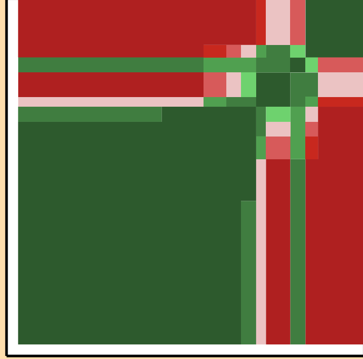
\sigma vs. E for ^{157}\text{Dy}(n,\text{inel.})
