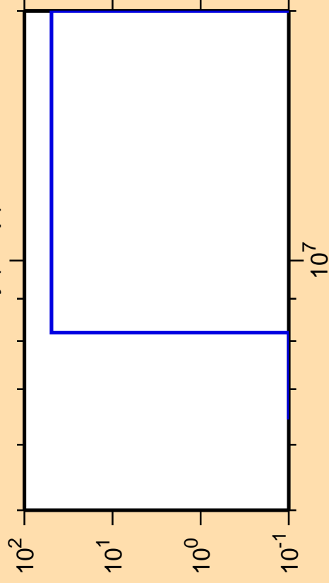
\Delta\sigma/\sigma vs. E for ^{157}\text{Dy}(n,np)
