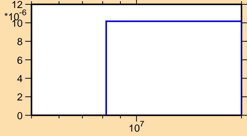
\sigma vs. E for ^{158}\text{Dy}(n,t)
