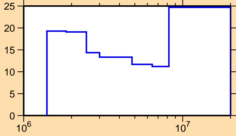
\Delta\sigma/\sigma vs. E for ^{158}\text{Dy}(n,n\text{cont.})
