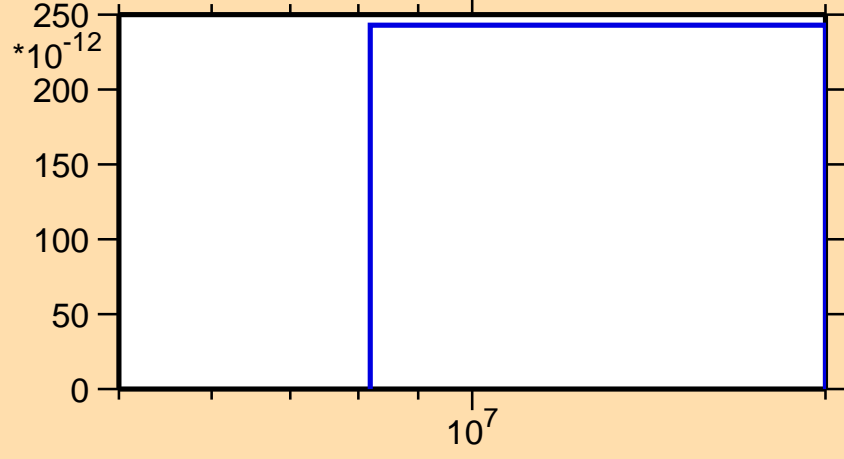
\sigma vs. E for ^{158}\text{Dy}(n,\text{nd})
