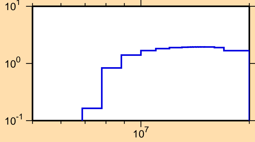
\sigma vs. E for ^{159}\text{Dy}(n,2n)
