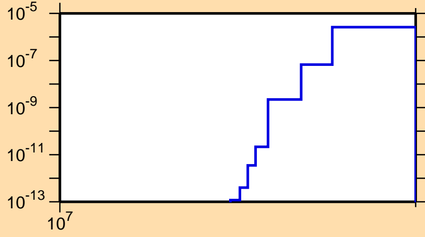
\sigma vs. E for ^{159}\text{Dy}(n,nd)
