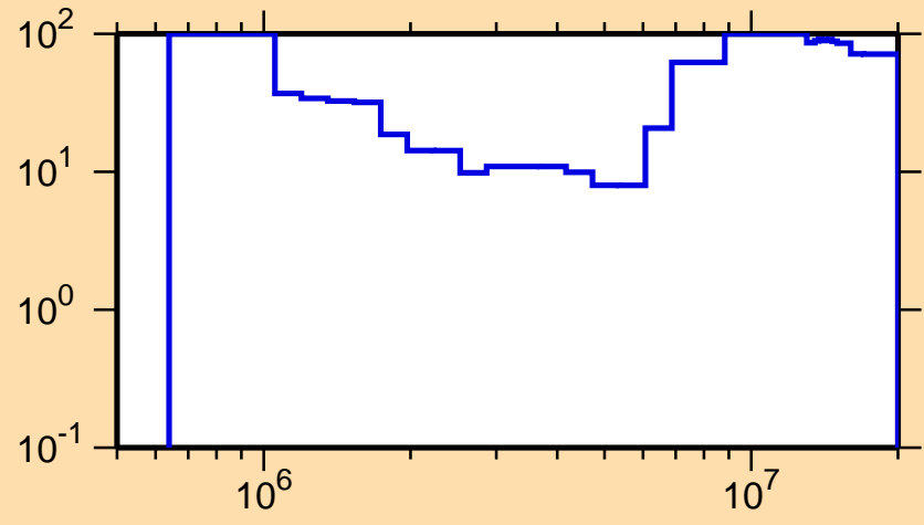
\Delta\sigma/\sigma vs. E for ^{159}\text{Dy}(n,n\text{cont.})
