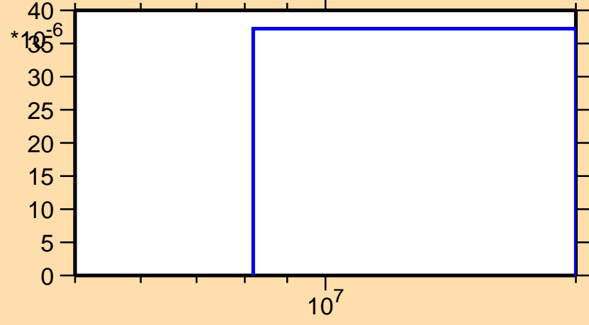
\sigma vs. E for ^{159}\text{Dy}(n,t)
