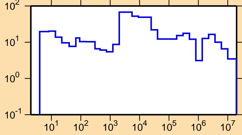
\Delta\sigma/\sigma vs. E for ^{160}\text{Dy}(n,\text{el.})
