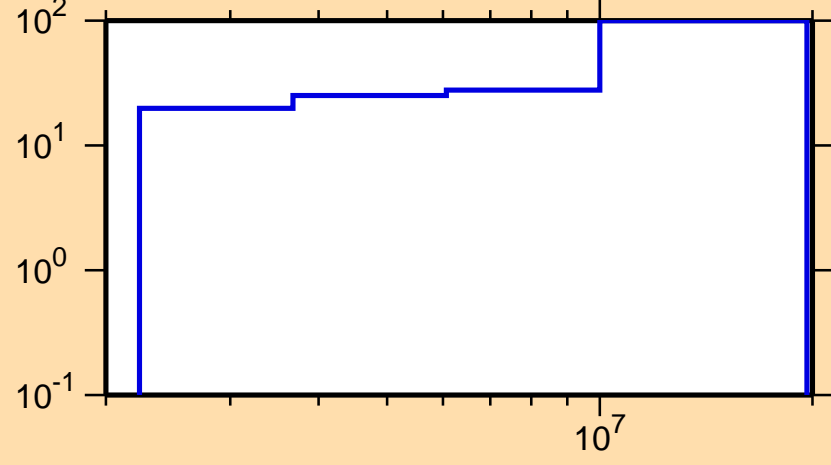
\Delta\sigma/\sigma vs. E for ^{160}\text{Dy}(n,\gamma)
