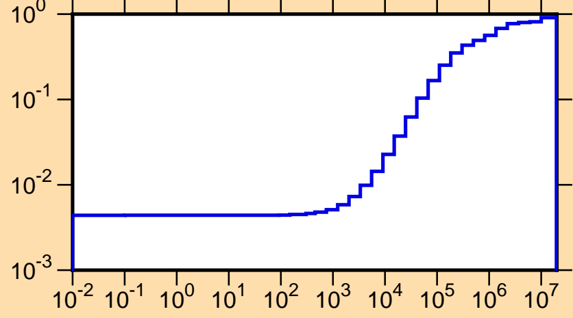
\mu vs. E for ^{161}\text{Dy}(\text{mt251})
