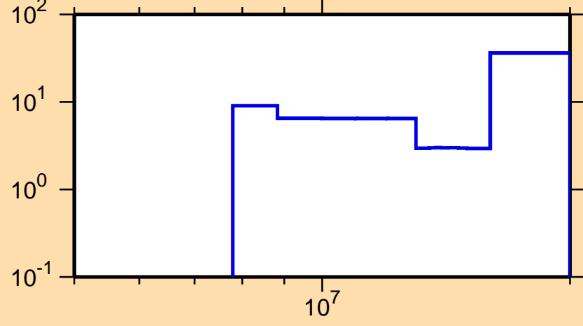
\Delta\sigma/\sigma vs. E for ^{162}\text{Dy}(n,2n)
