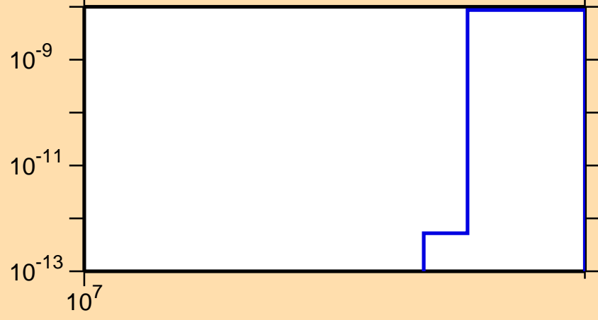
\sigma vs. E for ^{162}\text{Dy}(n,nt)
