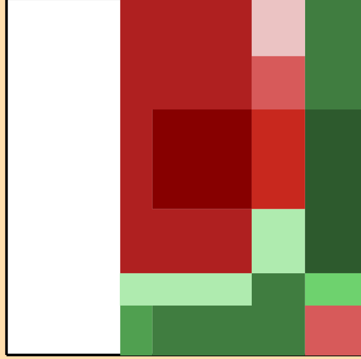
\Delta\sigma/\sigma vs. E for ^{162}\text{Dy}(n,2n)
