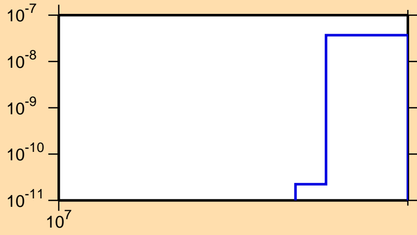
\sigma vs. E for ^{162}\text{Dy}(n,nd)
