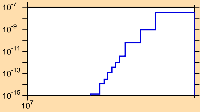
\sigma vs. E for ^{162}\text{Dy}(n,2n\alpha)
