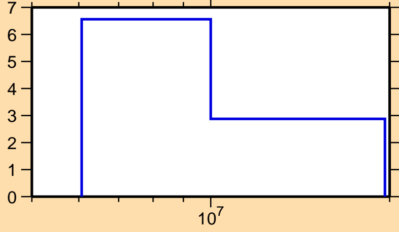
\Delta\sigma/\sigma vs. E for ^{162}\text{Dy}(n,2n)
