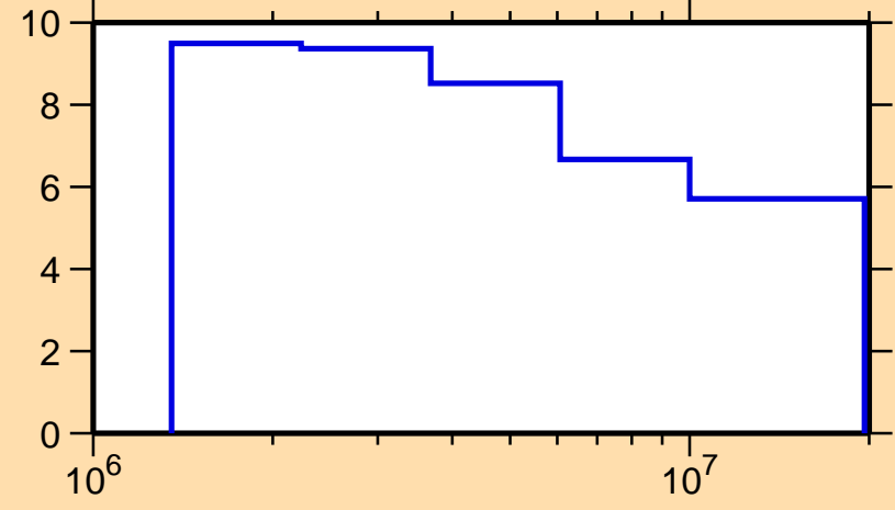
\Delta\sigma/\sigma vs. E for ^{162}\text{Dy}(n,n\text{nonel.})
