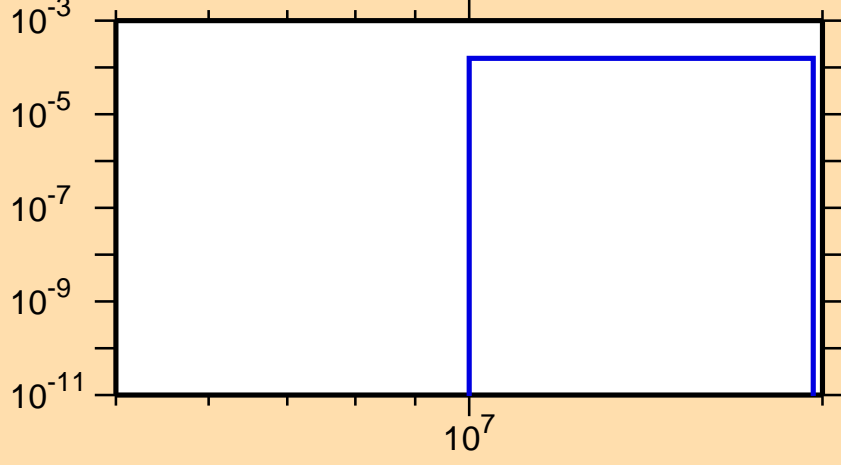
\sigma vs. E for ^{162}\text{Dy}(n,np)
