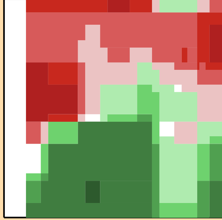
\Delta\sigma/\sigma vs. E for ^{163}\text{Dy}(n,n\text{cont.})
