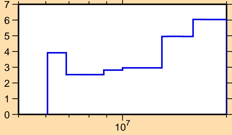
\Delta\sigma/\sigma vs. E for ^{163}\text{Dy}(n,\text{tot.})
