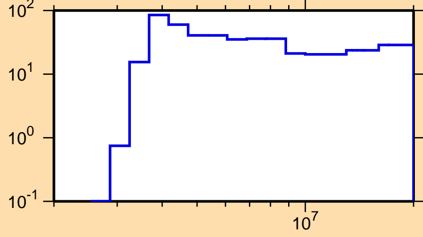
\Delta\sigma/\sigma vs. E for ^{163}\text{Dy}(n,p)
