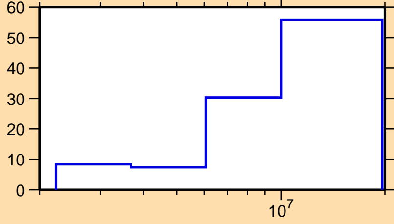
\Delta\sigma/\sigma vs. E for ^{163}\text{Dy}(n,ncont.)
