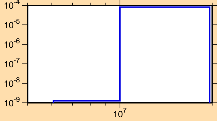
\sigma vs. E for ^{163}\text{Dy}(n,n\alpha)
