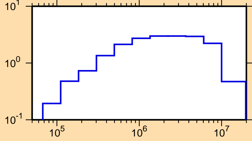
\sigma vs. E for ^{163}\text{Dy}(n,\text{inel.})
