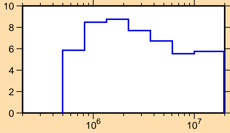
\Delta\sigma/\sigma vs. E for ^{163}\text{Dy}(n,n\text{onel.})
