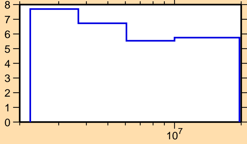
\Delta\sigma/\sigma vs. E for ^{163}\text{Dy}(n,\text{nonel.})
