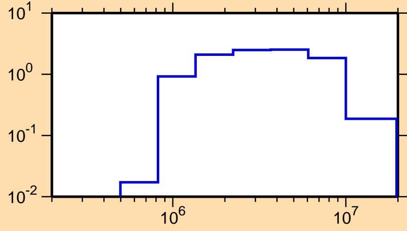
\sigma vs. E for ^{163}\text{Dy}(n,n\text{cont.})
