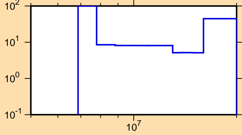
\Delta\sigma/\sigma vs. E for ^{164}\text{Dy}(n,2n)
