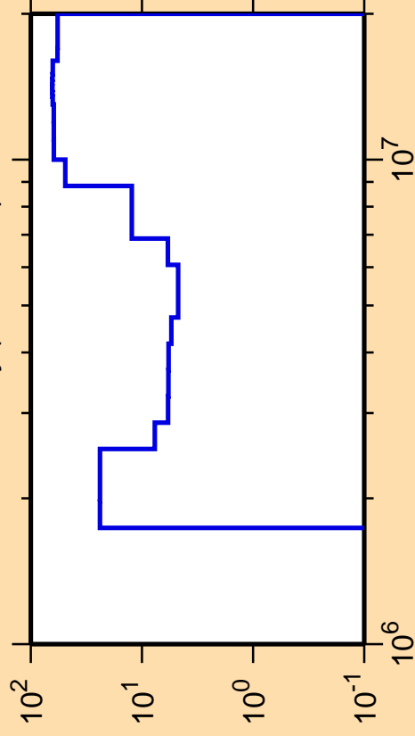
\Delta\sigma/\sigma vs. E for ^{164}\text{Dy}(n,\text{ncont.})
