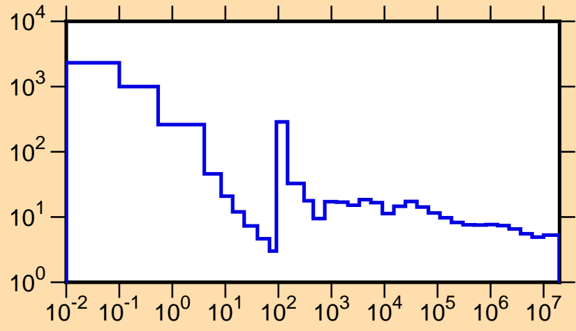
\sigma vs. E for ^{164}\text{Dy}(n,\text{tot.})
