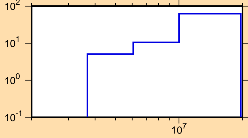
\Delta\sigma/\sigma vs. E for ^{164}\text{Dy}(n,ncont.)
