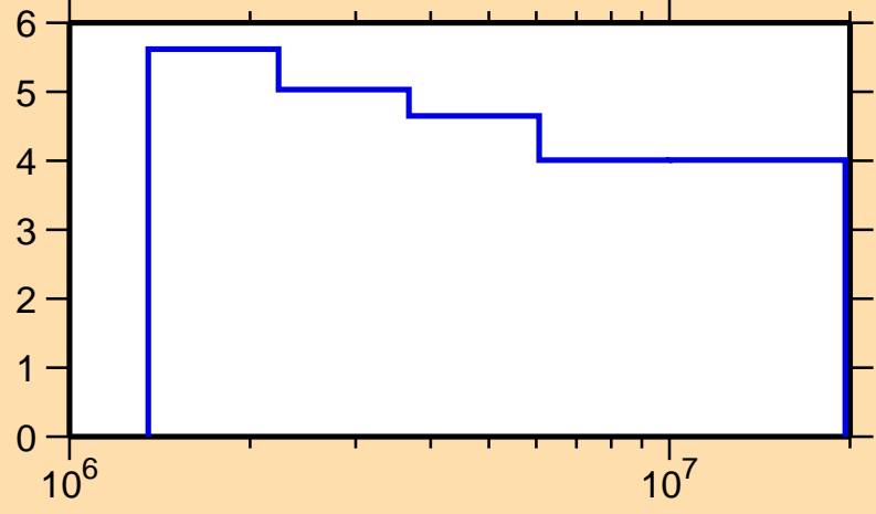
\Delta\sigma/\sigma vs. E for ^{164}\text{Dy}(n,n\text{nonel.})
