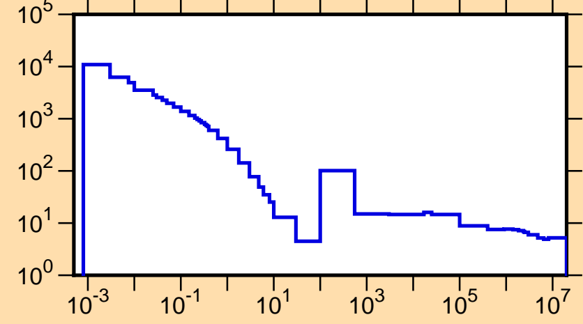
\sigma vs. E for ^{164}\text{Dy}(n,\text{tot.})
