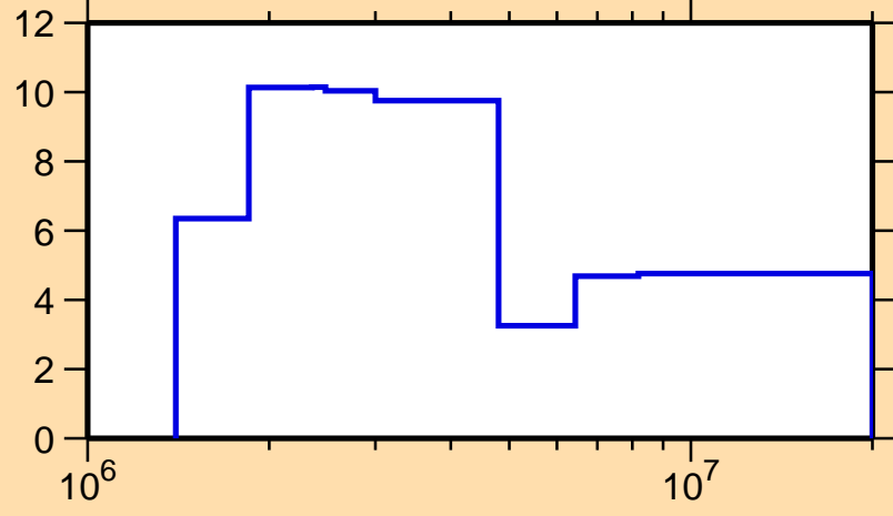
\Delta\sigma/\sigma vs. E for ^{164}\text{Dy}(n,el.)
