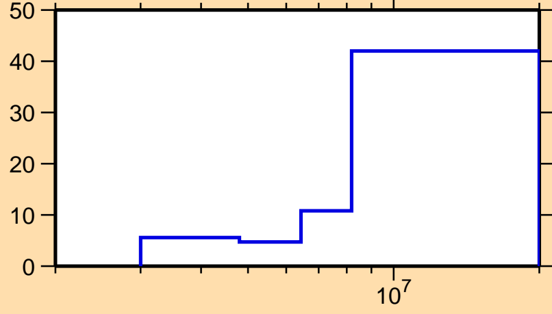
\Delta\sigma/\sigma vs. E for ^{164}\text{Dy}(n,ncont.)
