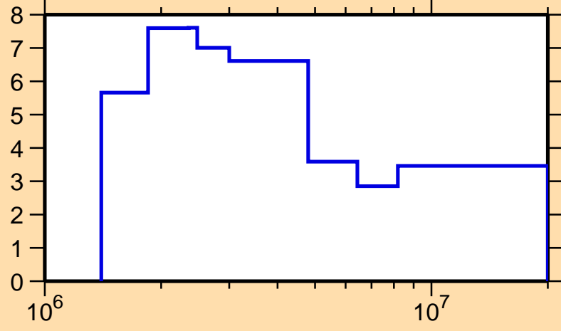
\Delta\sigma/\sigma vs. E for ^{164}\text{Dy}(n,tot.)
