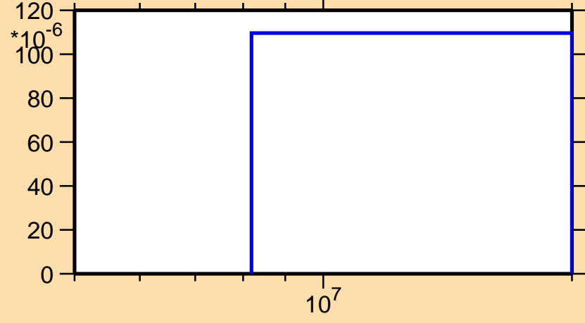
\sigma vs. E for ^{164}\text{Dy}(n,d)
