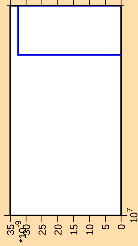
\Delta\sigma/\sigma vs. E for ^{165}\text{Dy}(\text{mt 11})
