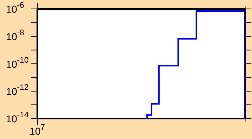
\sigma vs. E for ^{165}\text{Dy}(n,\text{nd})
