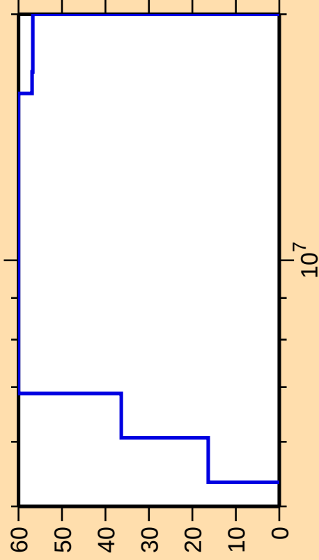
\Delta\sigma/\sigma vs. E for ^{165}\text{Dy}(n,n\text{cont.})
