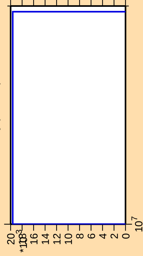
\Delta\sigma/\sigma vs. E for ^{165}\text{Dy}(n,\text{He}3)
