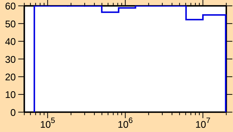
\Delta\sigma/\sigma vs. E for ^{165}\text{Dy}(n,n_1)
