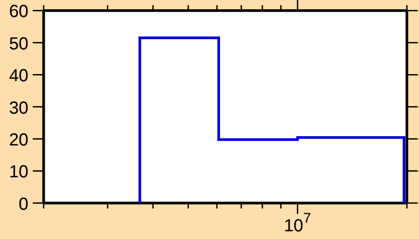
\Delta\sigma/\sigma vs. E for ^{165}\text{Dy}(n,2n)
