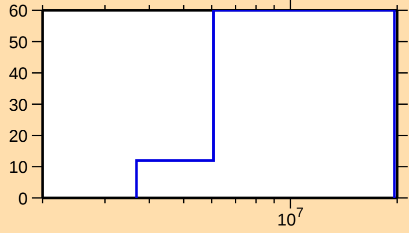
\Delta\sigma/\sigma vs. E for ^{165}\text{Dy}(n,ncont.)
