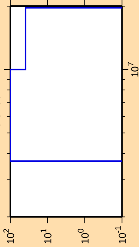
\Delta\sigma/\sigma vs. E for ^{165}\text{Dy}(n,p)
