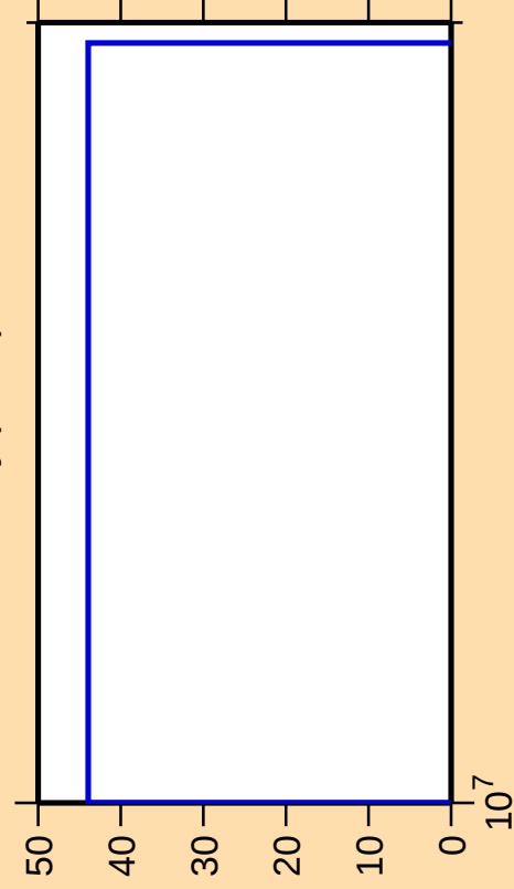
\Delta\sigma/\sigma vs. E for ^{165}\text{Dy}(n,3n)
