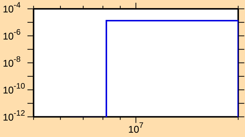
\sigma vs. E for ^{165}\text{Dy}(n,n\alpha)
