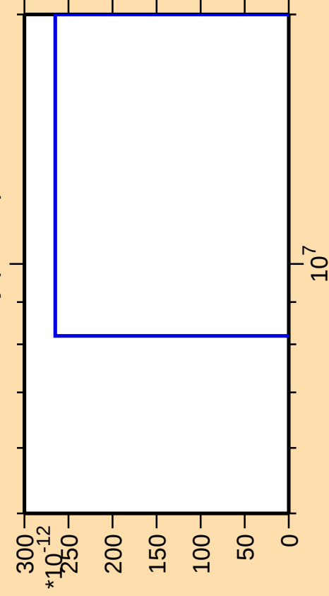
\Delta\sigma/\sigma vs. E for ^{165}\text{Dy}(\text{mt } 11)
