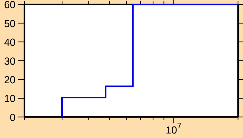
\Delta\sigma/\sigma vs. E for ^{165}\text{Dy}(n,n\text{cont.})
