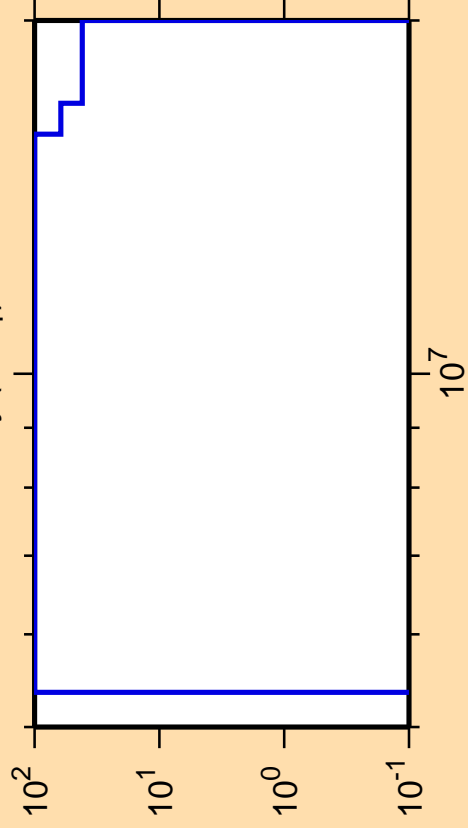
\Delta\sigma/\sigma vs. E for ^{165}\text{Dy}(n,n_1)
