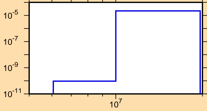
\sigma vs. E for ^{165}\text{Dy}(n,n\alpha)
