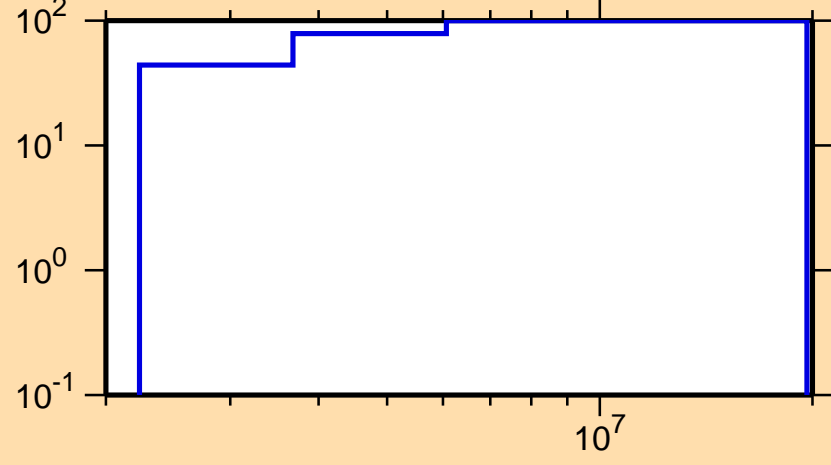
\Delta\sigma/\sigma vs. E for ^{165}\text{Dy}(n,n_1)
