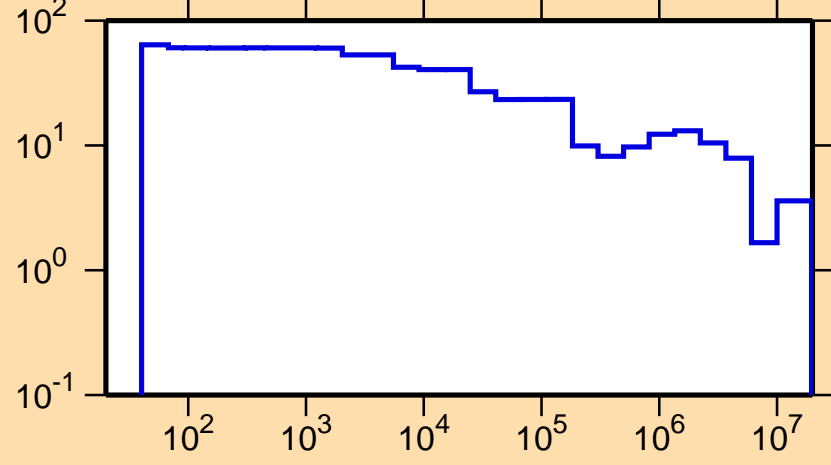
\Delta\sigma/\sigma vs. E for ^{165}\text{Dy}(n,\text{tot.})
