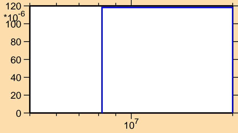
\sigma vs. E for ^{165}\text{Dy}(n,d)
