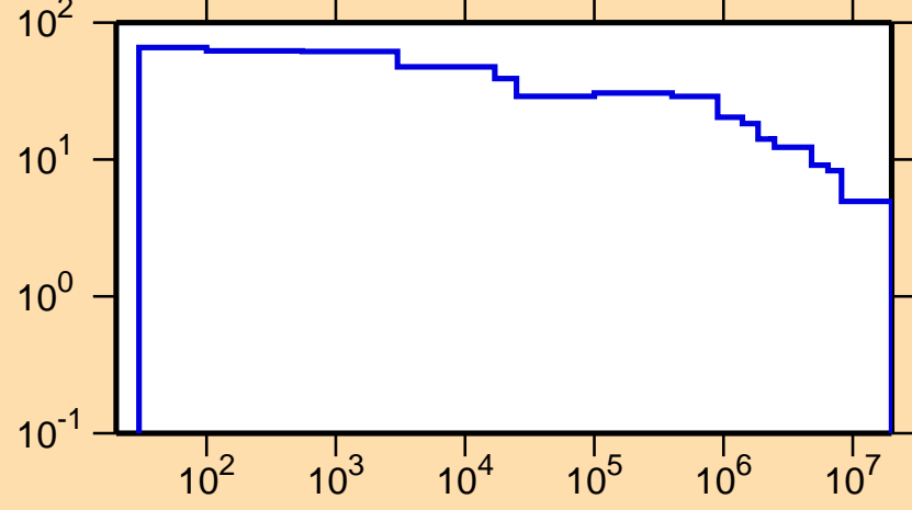
\Delta\sigma/\sigma vs. E for ^{165}\text{Dy}(n,\text{nonel.})
