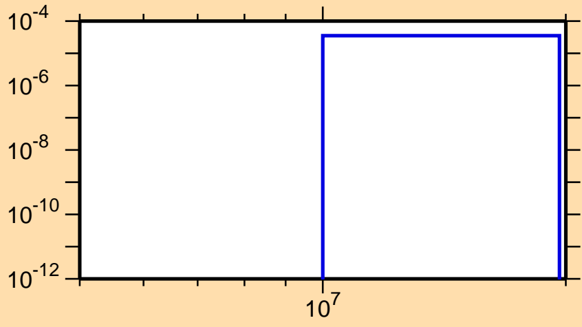
\sigma vs. E for ^{166}\text{Dy}(n,d)
