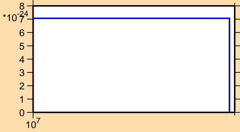
\sigma vs. E for ^{166}\text{Dy} (mt 11)
