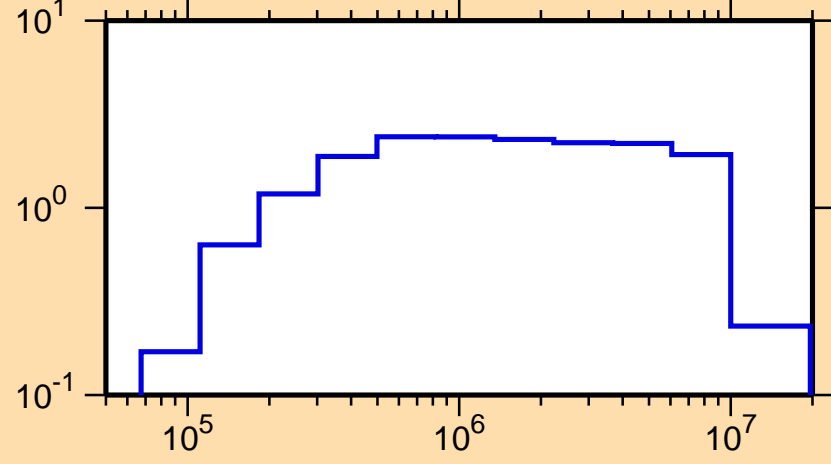
\sigma vs. E for ^{166}\text{Dy}(n,\text{inel.})
