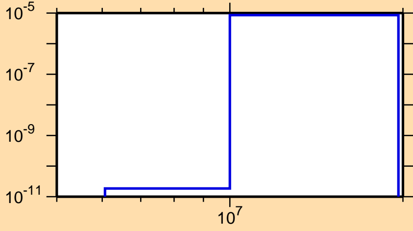
\sigma vs. E for ^{166}\text{Dy}(n,n\alpha)
