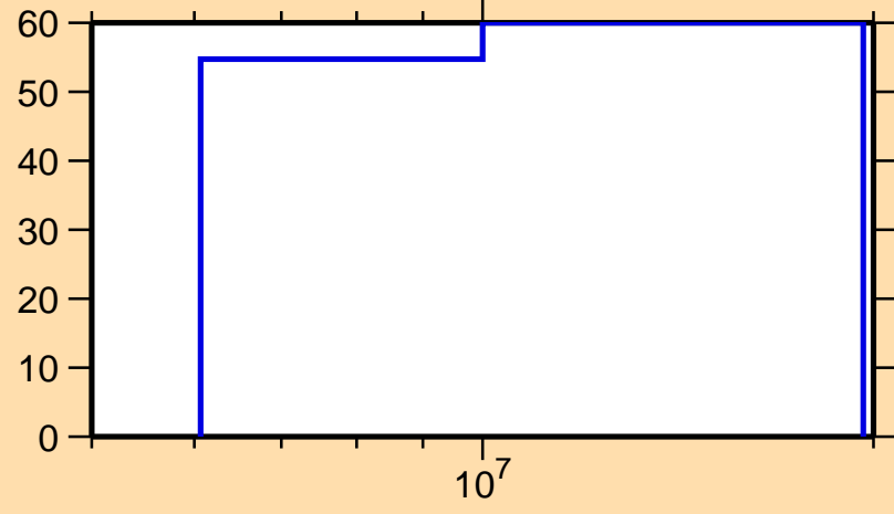
\Delta\sigma/\sigma vs. E for ^{166}\text{Dy}(n,ncont.)
