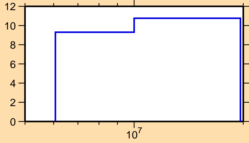
\Delta\sigma/\sigma vs. E for ^{166}\text{Dy}(n,el.)
