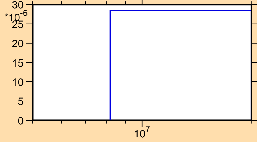
\sigma vs. E for ^{166}\text{Dy}(n,d)
