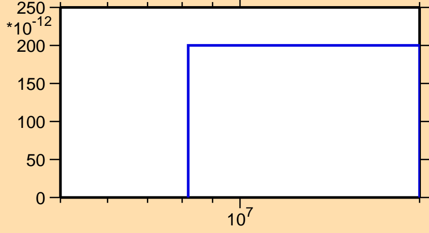
\sigma vs. E for ^{166}\text{Dy}(n,\text{nd})
