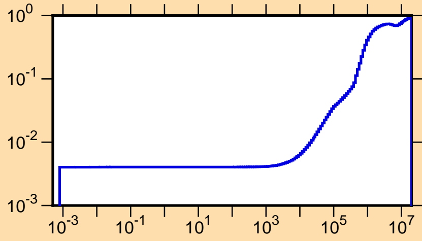
\mu vs. E for ^{167}\text{Dy}(\text{mt251})
