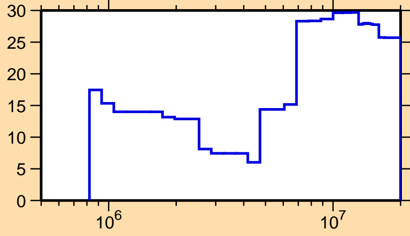
\Delta\sigma/\sigma vs. E for ^{167}\text{Dy}(n,inel.)
