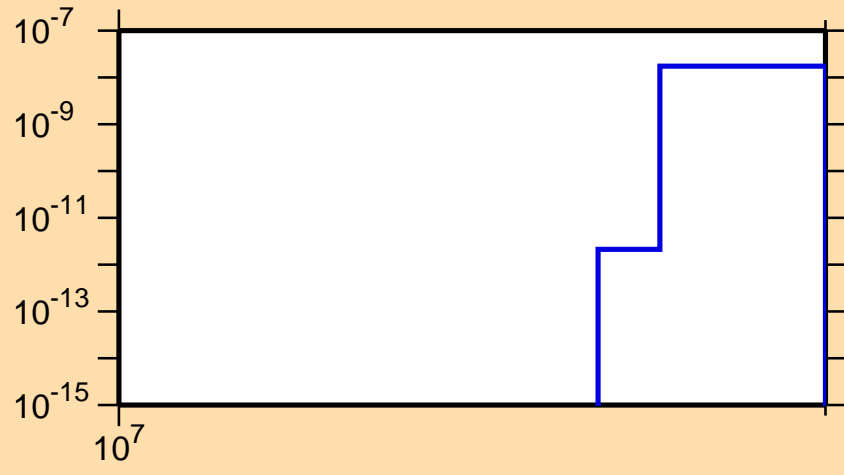
\sigma vs. E for ^{167}\text{Dy}(n,2np)
