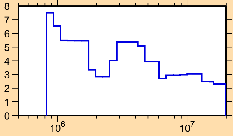
\Delta\sigma/\sigma vs. E for ^{167}\text{Dy}(n,tot.)
