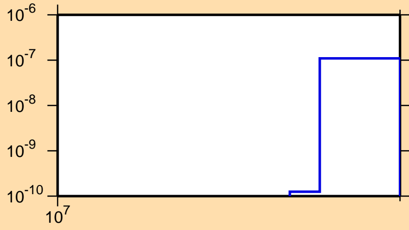
\sigma vs. E for ^{167}\text{Dy}(n,nt)
