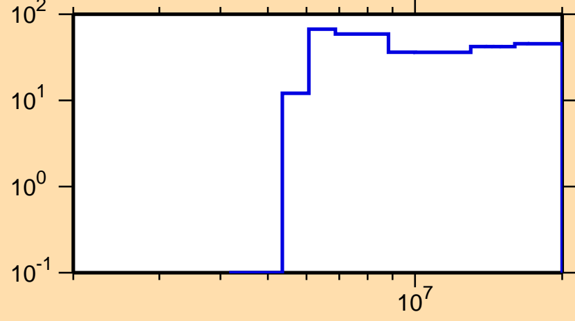
\Delta\sigma/\sigma vs. E for ^{167}\text{Dy}(n,p)
