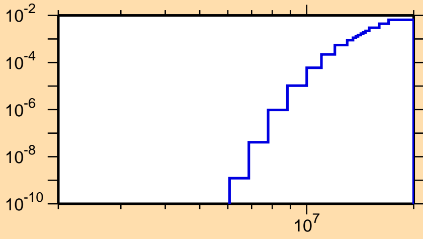
\sigma vs. E for ^{167}\text{Dy}(n,p)
