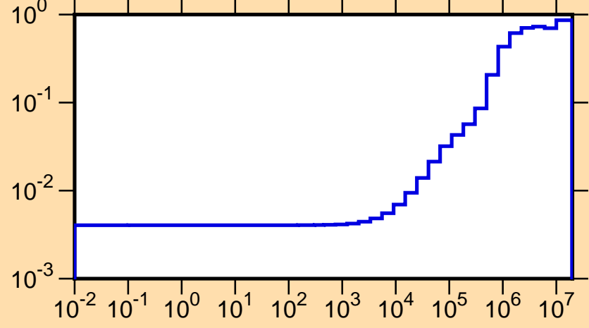
\mu vs. E for ^{167}\text{Dy}(\text{mt251})
