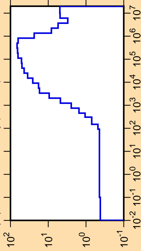
\Delta\mu/\mu vs. E for ^{167}\text{Dy}(\text{mt251})
