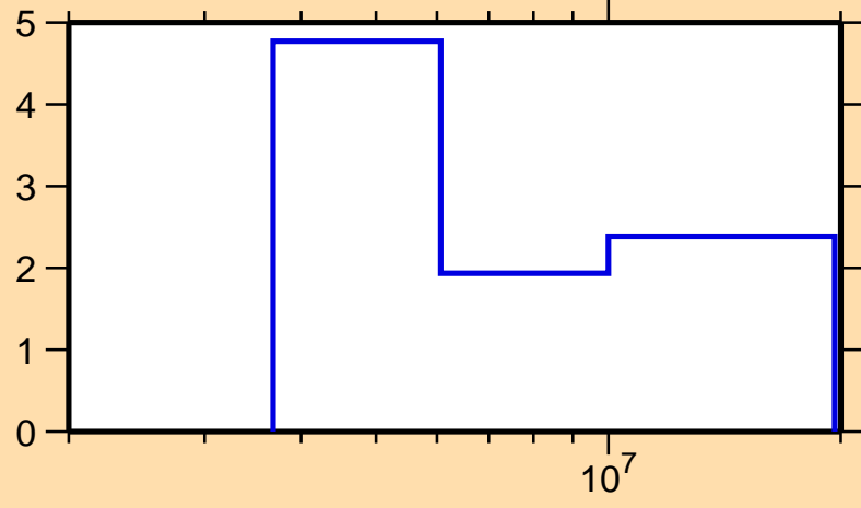
\Delta\sigma/\sigma vs. E for ^{167}\text{Dy}(n,\text{tot.})
