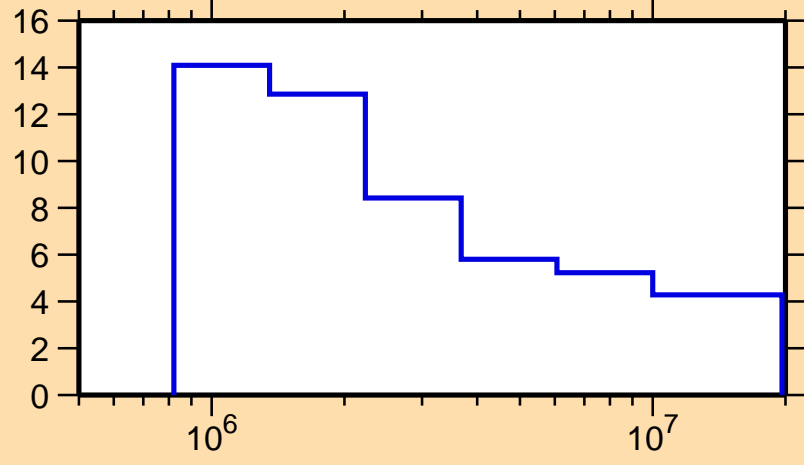
\Delta\sigma/\sigma vs. E for ^{167}\text{Dy}(n,n\text{onel.})
