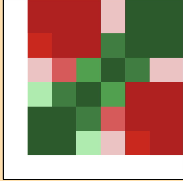
\sigma vs. E for ^{167}\text{Dy}(n,n\text{cont.})
