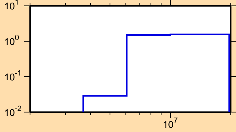
\sigma vs. E for ^{167}\text{Dy}(n,2n)
