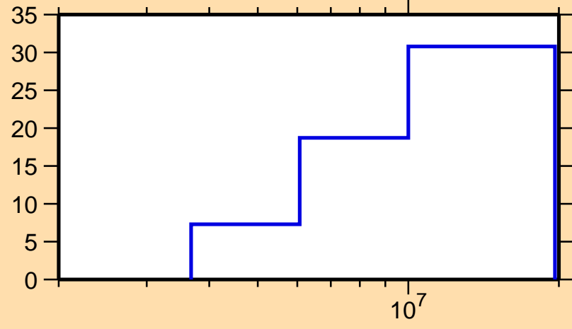
\Delta\sigma/\sigma vs. E for ^{167}\text{Dy}(n,ncont.)
