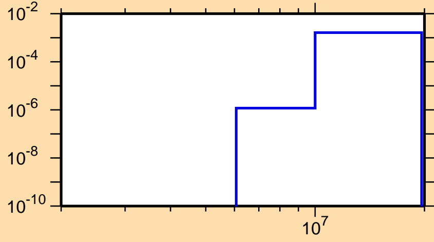
\sigma vs. E for ^{167}\text{Dy}(n,p)
