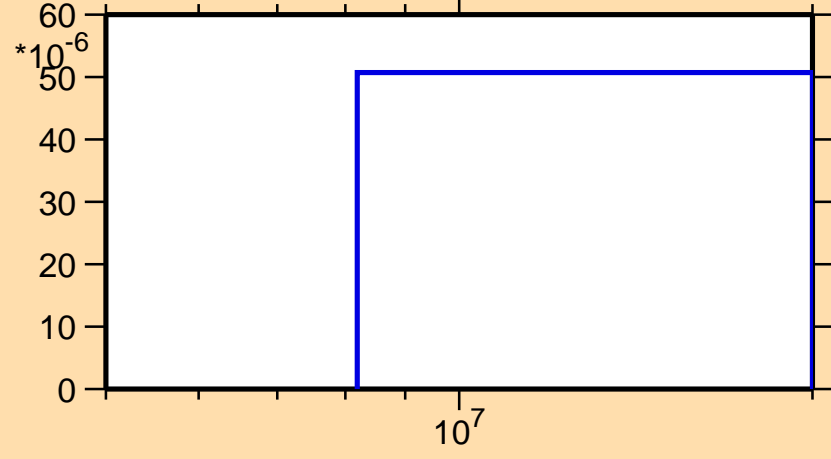
\sigma vs. E for ^{167}\text{Dy}(n,d)
