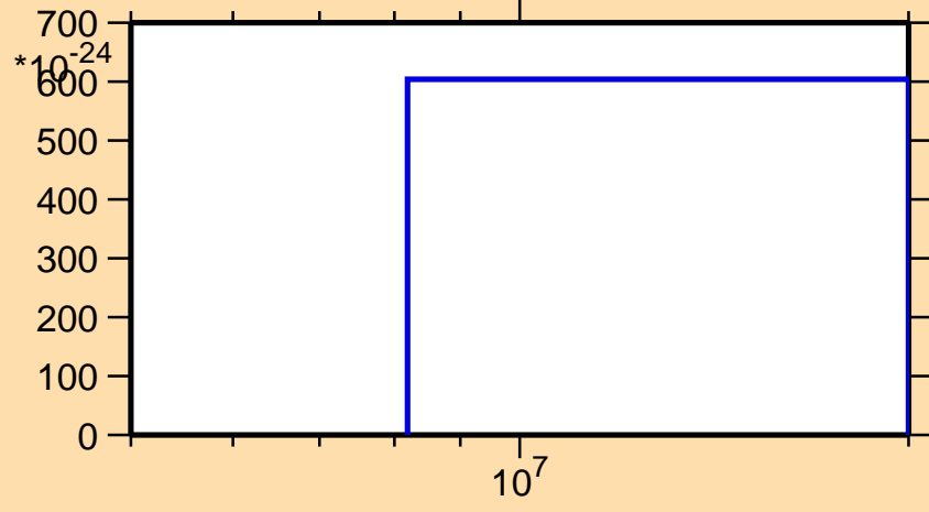
\sigma vs. E for ^{167}\text{Dy}(\text{mt } 11)
