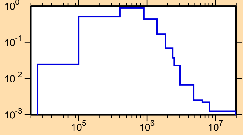
\sigma vs. E for ^{167}\text{Dy}(n,n_2)
