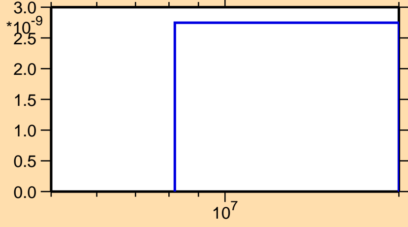
\sigma vs. E for ^{167}\text{Dy}(n,\text{nd})
