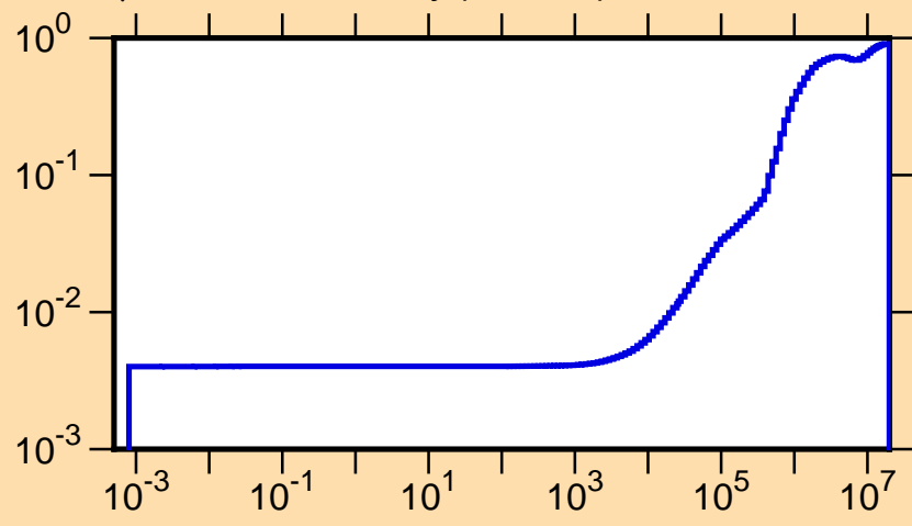
\mu vs. E for ^{168}\text{Dy}(\text{mt251})
