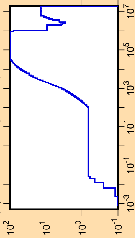
\Delta\mu/\mu vs. E for ^{168}\text{Dy}(\text{mt251})
