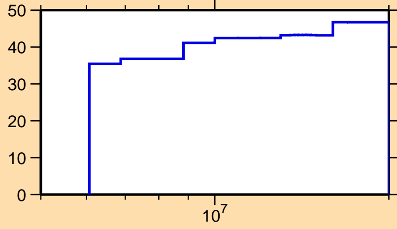
\Delta\sigma/\sigma vs. E for ^{168}\text{Dy}(n,n_1)
