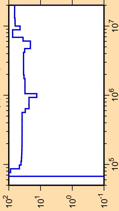
\Delta\sigma/\sigma vs. E for ^{168}\text{Dy}(n,\text{inel.})
