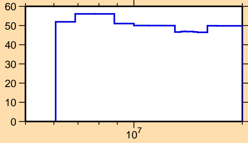
\Delta\sigma/\sigma vs. E for ^{168}\text{Dy}(n,el.)
