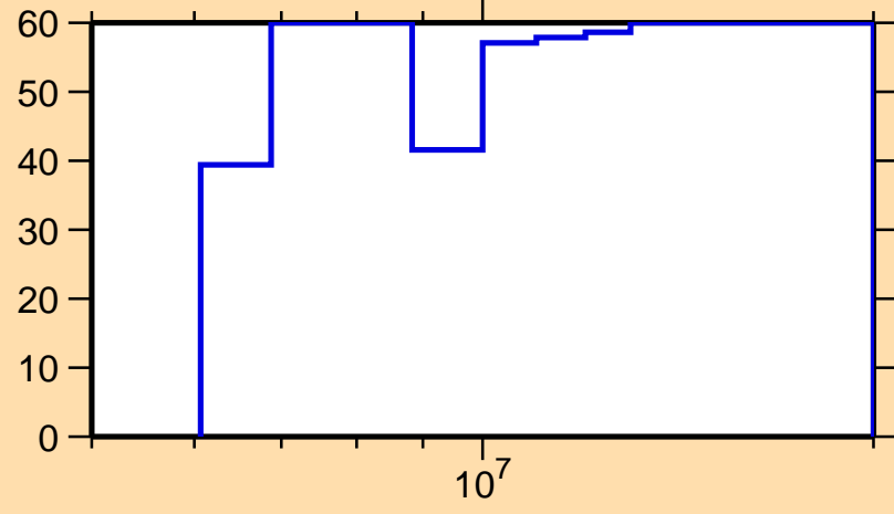
\Delta\sigma/\sigma vs. E for ^{168}\text{Dy}(n,ncont.)
