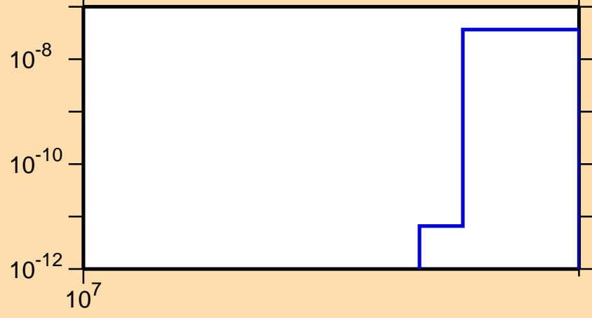
\sigma vs. E for ^{168}\text{Dy}(n,nt)
