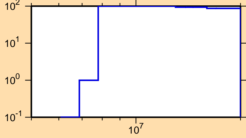
\Delta\sigma/\sigma vs. E for ^{168}\text{Dy}(n,p)
