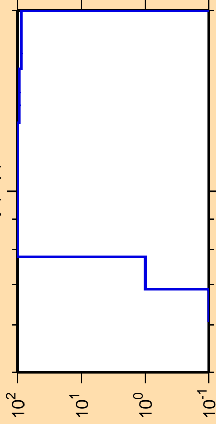
\Delta\sigma/\sigma vs. E for ^{168}\text{Dy}(n,p)
