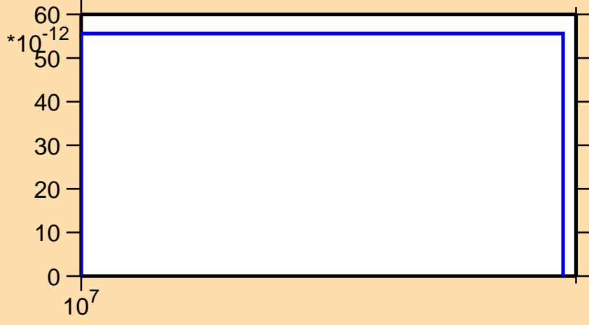
\sigma vs. E for ^{168}\text{Dy}(n,\text{nd})
