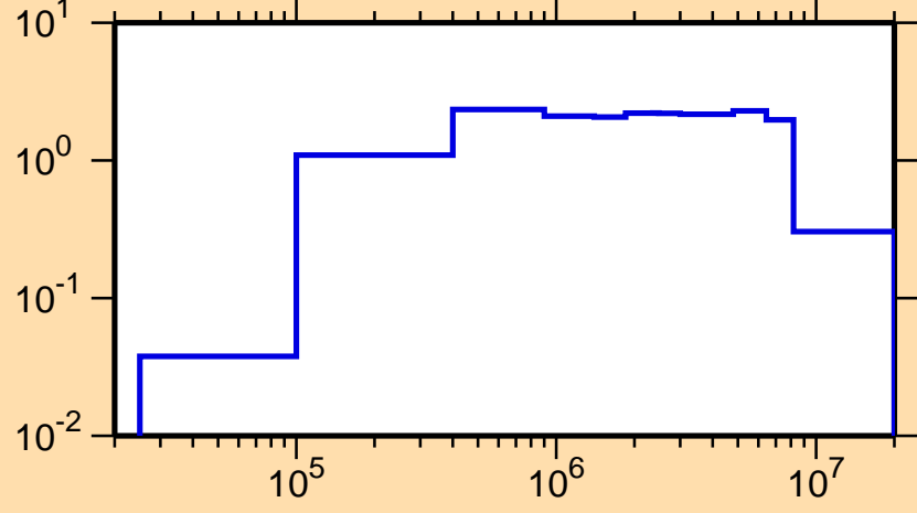
\sigma vs. E for ^{168}\text{Dy}(n,\text{inel.})
