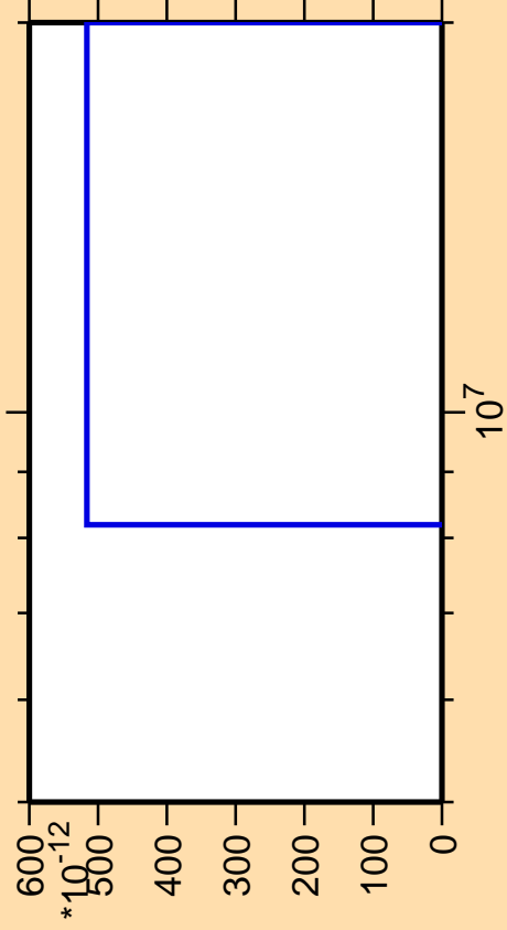
\Delta\sigma/\sigma vs. E for ^{168}\text{Dy}(\text{mt } 11)
