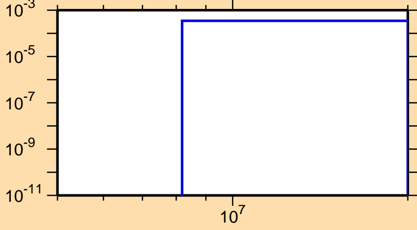
\sigma vs. E for ^{168}\text{Dy}(n,p)
