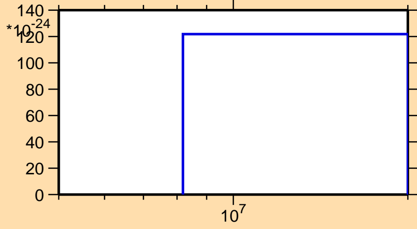
\sigma vs. E for ^{168}\text{Dy}(\text{mt } 11)
