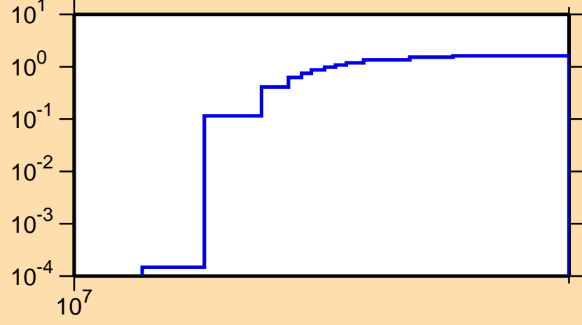
\sigma vs. E for ^{169}\text{Dy}(n,3n)
