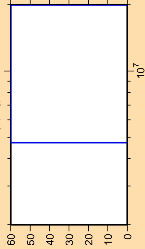
\Delta\sigma/\sigma vs. E for ^{169}\text{Dy}(n,\gamma)
