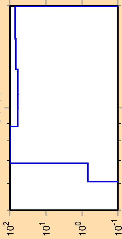
\Delta\sigma/\sigma vs. E for ^{169}\text{Dy}(n,p)
