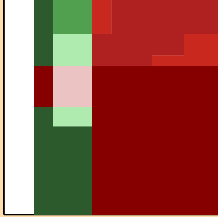
\Delta\sigma/\sigma vs. E for ^{169}\text{Dy}(n,p)
